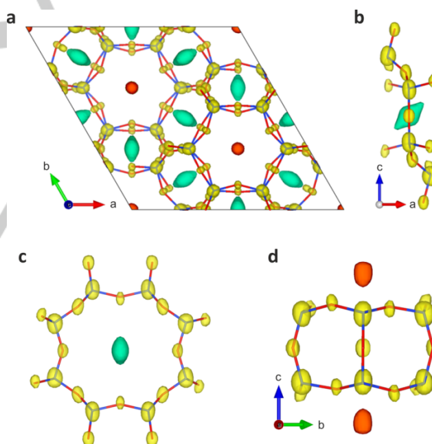
Figure 4. Structure solution. Electrostatic potential map obtained from ab initio structure solution using single nanocrystals PEDT datasets. Isosurface levels correspond to 3.5σ[V(r)]. a , Projection along c . Yellow, red and green transparent colours indicate framework, SII and SIII' sites, respectively. Tetrahedral sites (blue lines) and framework oxygen atoms (red lines) are included for clarity. b , Side view of eight membered ring (8MR) with elongated potential around SIII' site. c , Perpendicular view of 8MR. d , Side view of D6R with SII sites.
