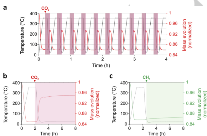
Figure 3. CO 2 vs CH 4 absorption. a , Thermogravimetric analysis (TGA) of nanosized CHA zeolite subjected to 10 consecutive adsorption/desorption cycles of CO 2 : temperature variation (black line), CO 2 sorption (red rectangles) and mass variation (red line). b , mass variation upon CO 2 adsorption (red line) and (c) CH 4 adsorption (green line) on as-synthesized nanosized CHA. The CH 4 flow was delayed and started at 25 °C instead of 350 °C for safety reasons.
