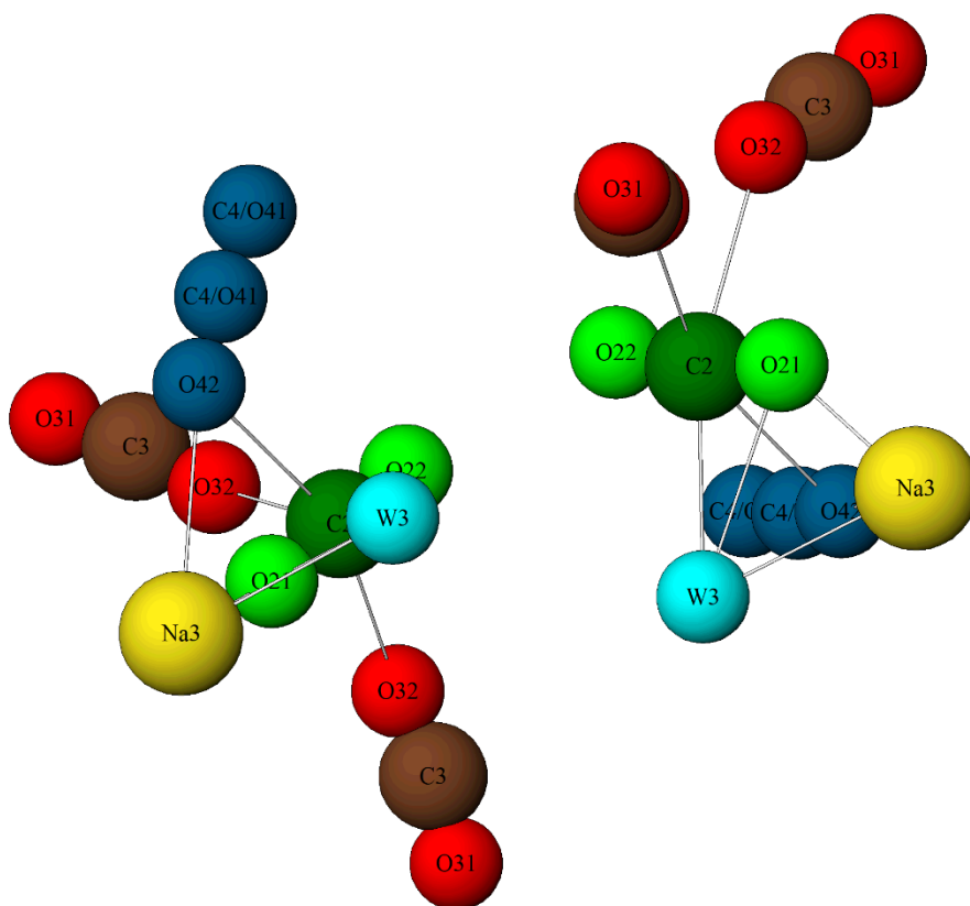
Figure 6. Possible distribution of CO 2 molecules, Na cations and W3 molecule in the supercage of the Na-Y-CO 2 sample (only Na3 and W3 bonded to the clusters are drawn). The labels C2, O21 and O22 represent the CO 2 -2 molecule, C3, O31 and O32 the CO 2 -3 molecule and C4, O41 and O42 the CO 2 -4 one.
