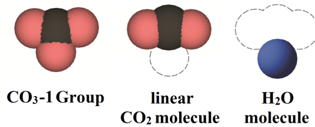
Figure 4. Possible configurations of the \text{CO}_3 -1 group in Na-X- \text{CO}_2 sample.
