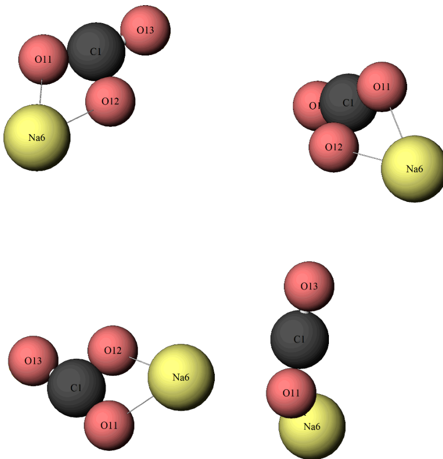
Figure 5. Possible distribution of \text{CO}_3 groups and Na6 cations in the superpage of the Na-X- \text{CO}_2 sample, taking into account their occupancy factors and distances (only bonded Na6 are drawn).
