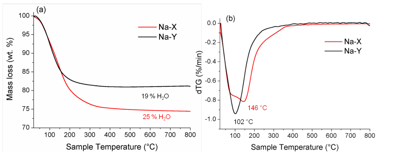
Figure 2. (a) Thermogravimetric (TG) and (b) differential thermogravimetric (dTG) curves of Na-X and Na-Y zeolite samples.
