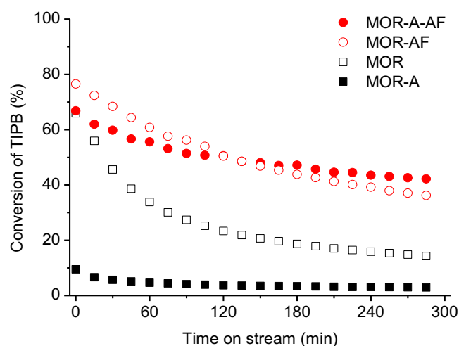
Figure 10. Conversion of 1,3,5-triisopropylbenzene as a function of the catalyst time on stream on MOR (open square), MOR-A (solid square), MOR-AF (open circle), and MOR-A-AF (solid circle). T = 350\text{ }^{\circ}\text{C} , P = 0.101\text{ MPa} , W/F_0 = 95\text{ kg}\cdot\text{s}\cdot\text{mol}^{-1} .
