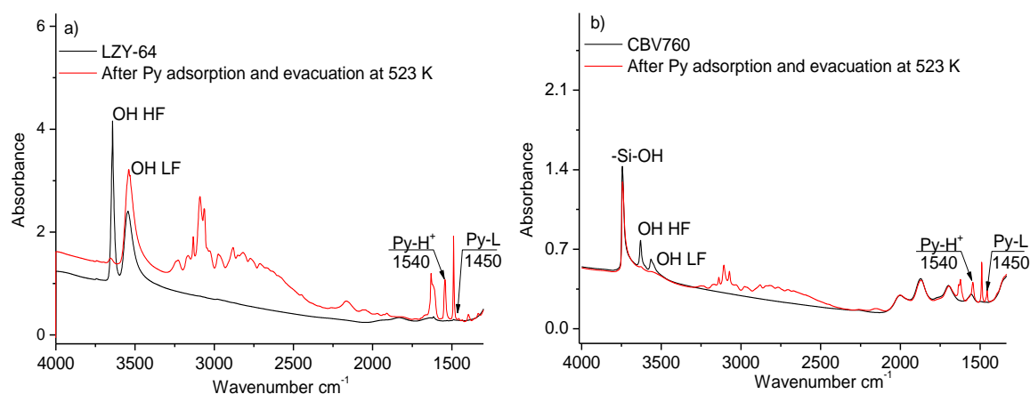
Figure 1. IR spectra before and after adsorption of pyridine and evacuation at 523 K under vacuum: a) LZY-64 and b) CBV760.
