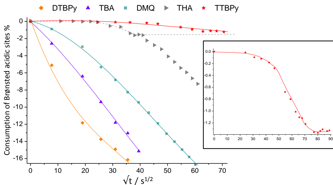
Figure 4. Consumption of the LZY-64 Brønsted acidity as a function of the square root of exposure time, \sqrt{t} , at 298 K for various basic probe molecules (inset: zoom on TTBPy).
