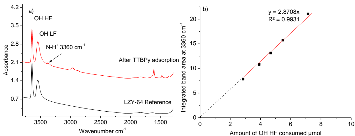
Figure 6. a) IR spectra of LZY-64 before and after 120 min contact with TTBPY vapor at 298 K, b) integrated intensity of the 3360 cm -1 band as a function of OH HF consumed.
