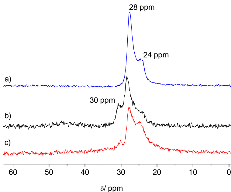
Figure 9. ^{31}\text{P} MAS NMR spectra of TPhPO a) pure, b) adsorbed on LZY-64, c) adsorbed on CBV760
