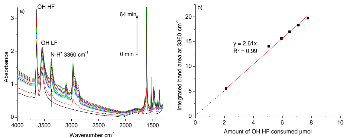
Figure 3. a) Time evolution of the IR spectra of LZY-64 in contact with 2,6 DTBPy, b) integrated band area at 3360\text{ cm}^{-1} as a function of the \text{OH}_{\text{HF}} consumed.
