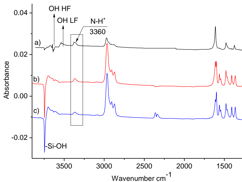
Figure 7. IR spectra of TTBPY adsorbed at 298 K and evacuated under vacuum at room temperature for 15 min on a) LZY-64, b) CBV720, c) CBV760.
