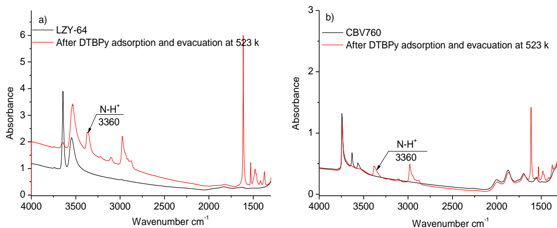
Figure 2. IR spectra before and after adsorption of 2,6 Di-tert-butylpyridine (DTBPy) and after evacuation at 523 K under vacuum: a) LZY-64 and b) CBV760.
