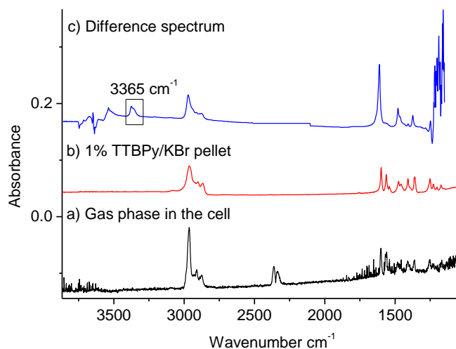
Figure 5. IR spectra of a) gas phase (TTBPY) in the cell (x 40), b) 1% TTBPY/KBr pellet, c) difference spectrum between TTBPY adsorbed on LZY-64 and the pristine LZY-64 (298 K).
