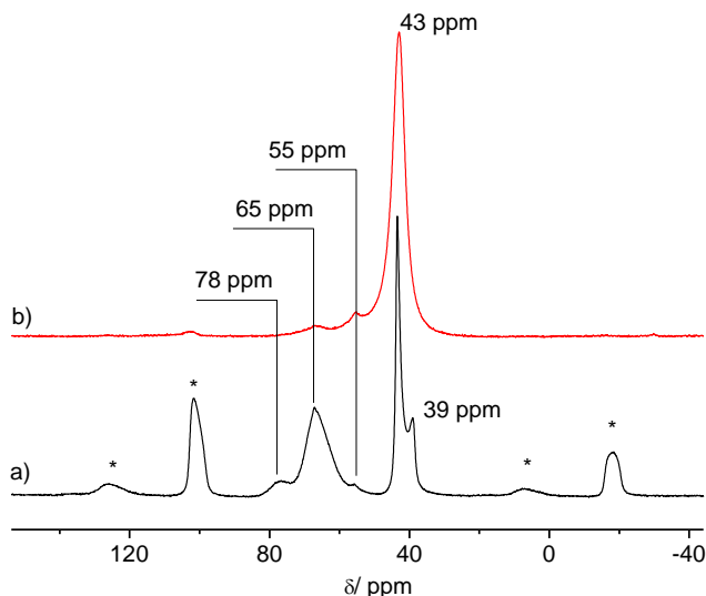
Figure 8. ^{31}\text{P} MAS NMR spectra of TMPO adsorbed on a) LZY-64, b) CBV760 (*: spinning side bands).
