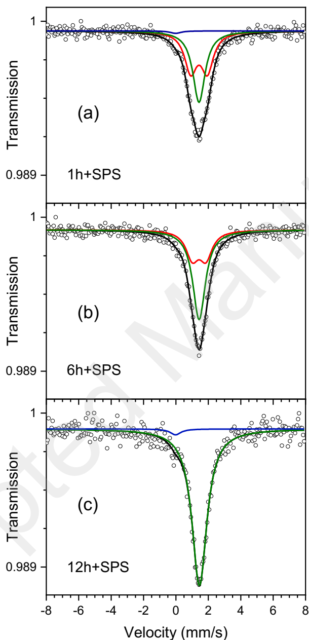
Figure 4. ^{119}\text{Sn} Mössbauer spectra at 295 K of (a) 1h+SPS, (b) 6h+SPS and (c) 12h+SPS samples.
