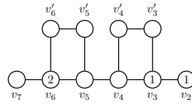
(b) After the first move: a cop moved from v_7 to v_6 .
