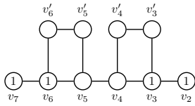
(a) Initial positions for cops in subgraph.
