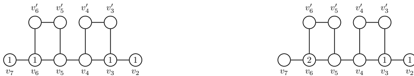
(a) Initial positions for cops in subgraph. (b) After the first move: a cop moved from v_7 to v_6 .
