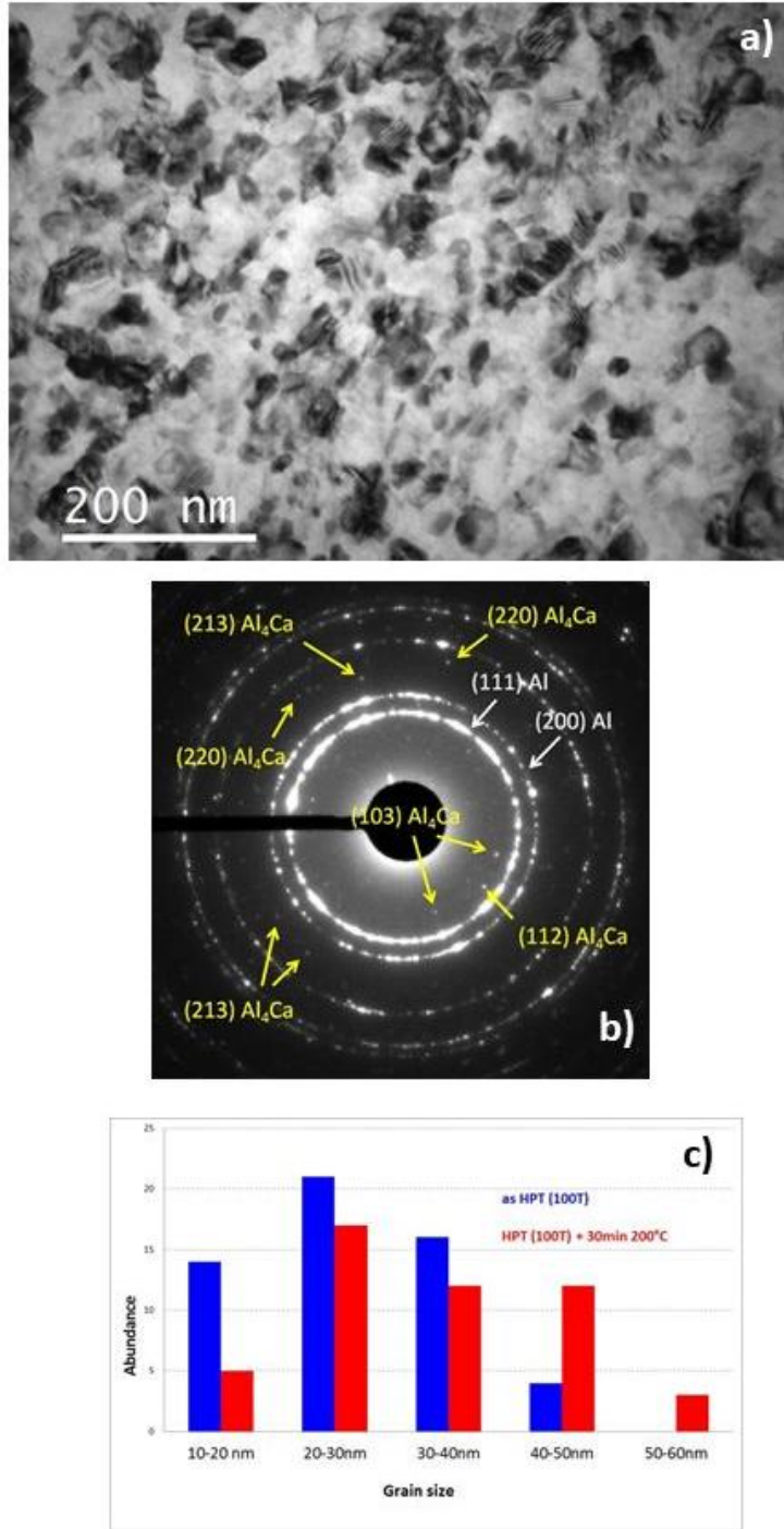
Figure 8: (a) TEM BF image showing the nanoscaled structure after in-situ annealing 30 min at 200 °C and (b) corresponding SAED pattern showing diffraction spots attributed to fcc Al and \text{Al}_4\text{Ca} phase. (c) Grain size distribution measured after 30 min at 200 °C and compared to the initial state.
