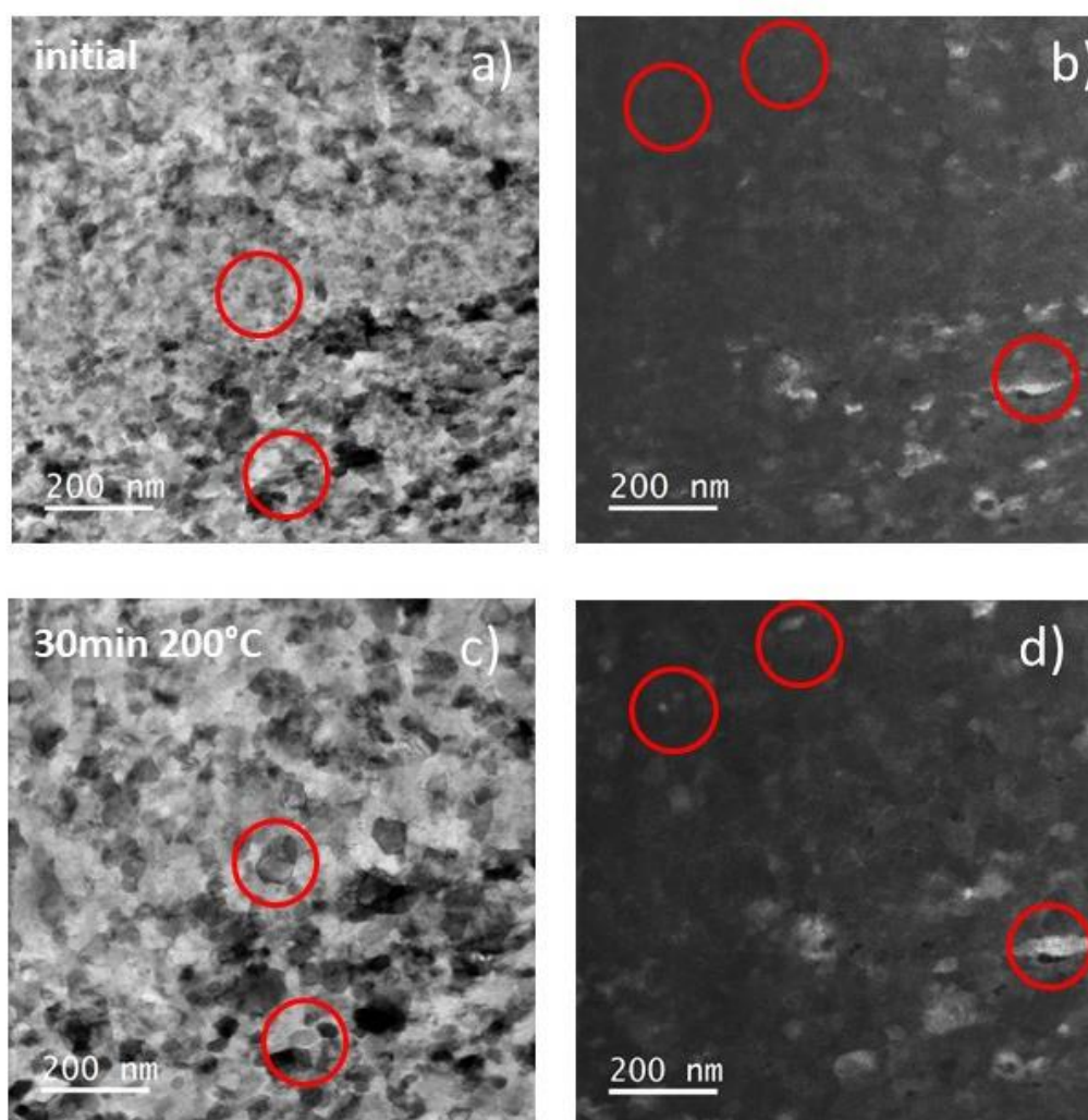
Figure 7: STEM BF (a, c) and HAADF (b, d) images of the nanoscale structure of the Al-Ca composite processed by 100 revolutions by HPT showing the microstructure evolution during in-situ annealing. The same regions are displayed in the initial state (a, b) and after 30 min at 200 °C (c, d). Grain growth and precipitation of Ca-rich clusters are highlighted by the red circles.
