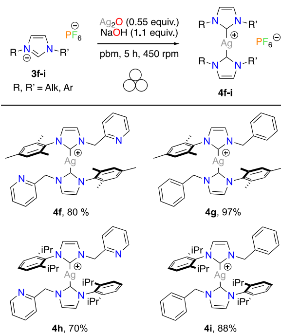
Scheme 3. Mechanochemical synthesis of homoleptic [Ag(NHC) 2 ]PF 6 complexes bearing N -alkyl, N -aryl ligands
