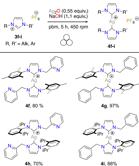
Scheme 3. Mechanochemical synthesis of homoleptic [Ag(NHC) 2 ]PF 6 complexes bearing N -alkyl, N -aryl ligands
