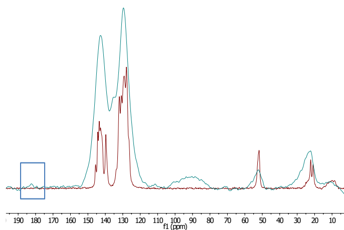
Figure 1. 13 C solid state HR-MAS NMR of IPr * ·HPF 6 3e (red) and [Ag(IPr * ) 2 ]PF 6 4e (blue)
