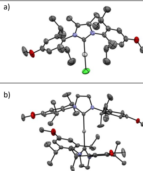
Figure 2. ORTEPs (at 50% probability level) of compounds (a) 2b , (b) 4a . Hydrogen atoms and PF 6 anion are omitted for clarity.
