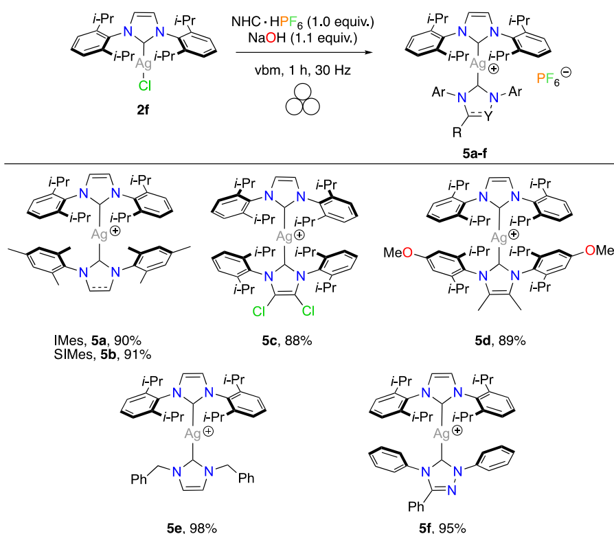
Scheme 4. Mechanochemistry of cationic heteroleptic silver complexes
