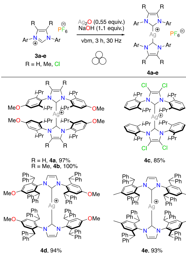
Scheme 2. Mechanosynthesis of homoleptic [\text{Ag}(\text{NHC})_2]\text{PF}_6 complexes bearing highly encumbered NHC ligands
