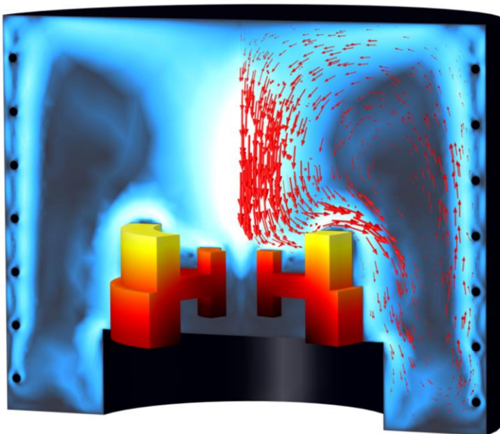
Muffle furnace heating
