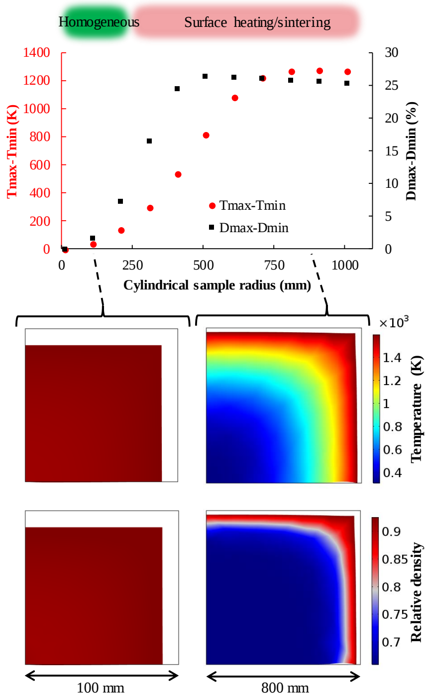
Fig.13 Scale effect on the temperature/relative density homogeneity; a cylindrical sample with same radius and height is surface heated for different size from 10mm to 1m; the maximum and minimum temperatures and relative densities differences ( T_{max}-T_{min} and D_{max}-D_{min} ) are compared for each size.
