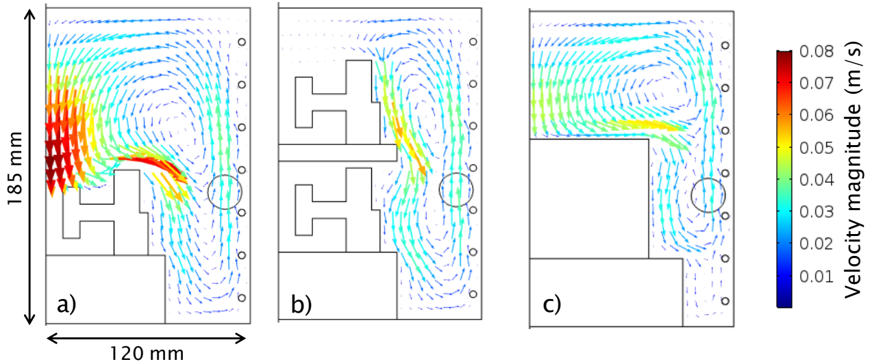
Fig.6 Convective velocity distribution for the a) gear, b) two gears and c) cylinder configurations.
