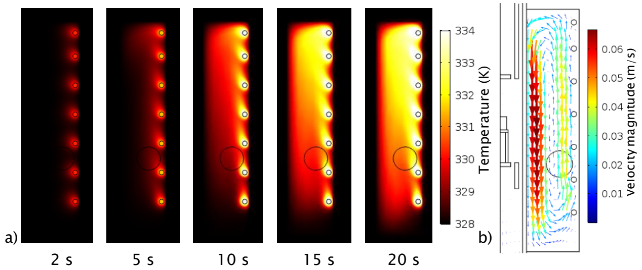
Fig.3 Dilatometer initial heating, a) temperature, b) convection velocity field.
