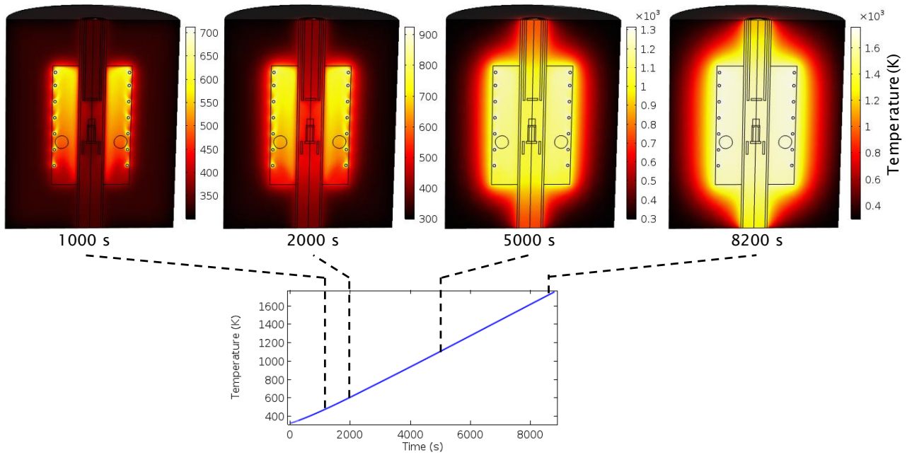
Fig.4 Dilatometer temperature distribution.
