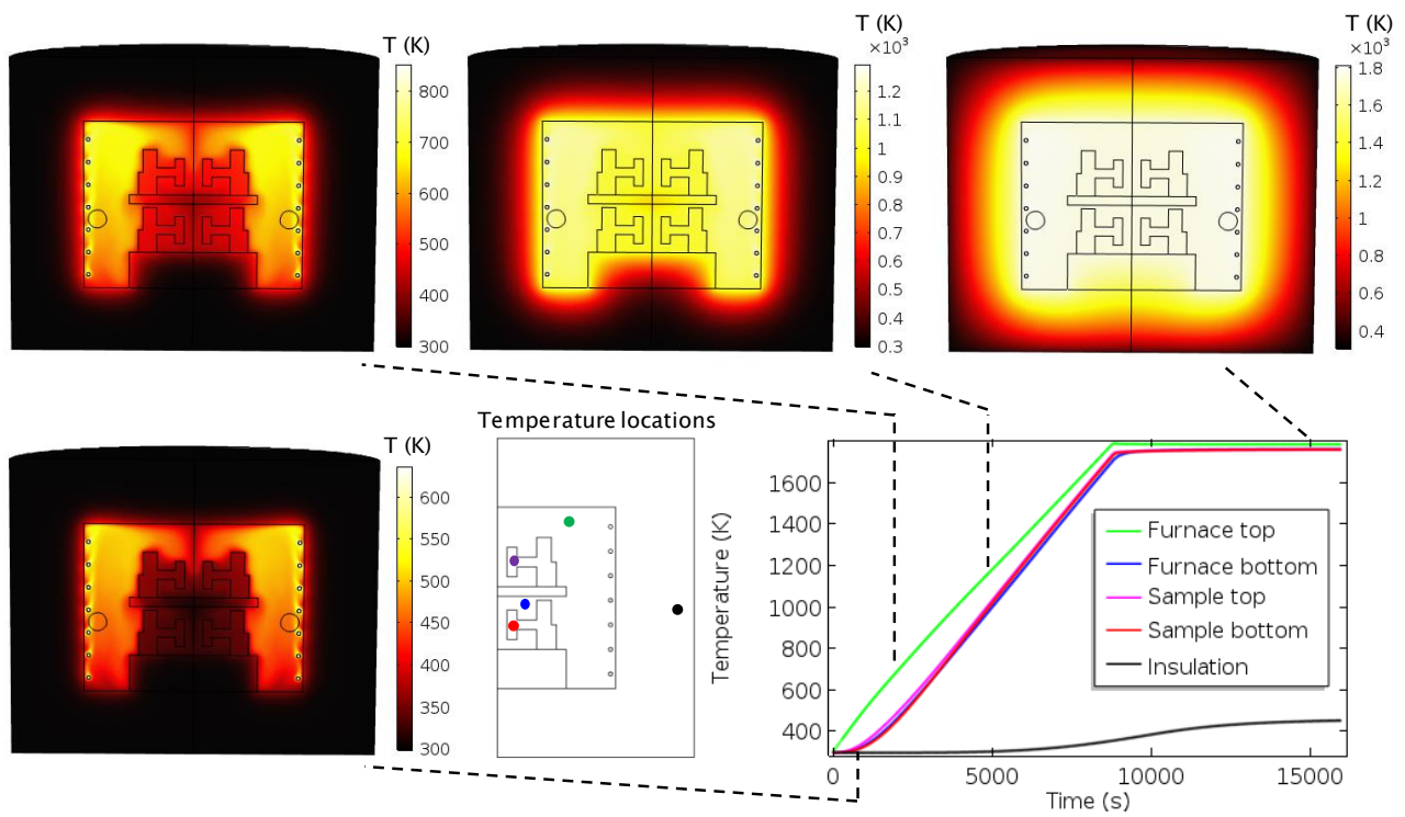
Fig.9 Temperature distribution for the two gear configuration.
