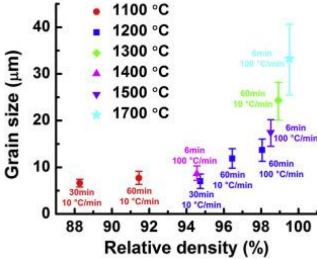
Fig. 5. Grain size as a function of the relative density of ZrN powder pellets obtained by SPS under 60 MPa.
