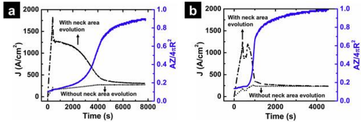
Fig. 4. Current density evolution with (black dash-dot line) and without (black dot line) consideration of the neck area change during the whole SPS cycle. Neck area evolution is shown with respect to the right y-axis (blue solid line). (a) SPS, 1200 °C, 60 MPa and 10 °C/min and (b) SPS, 1200 °C, 60 MPa and 100 °C/min. Electric current through the sample ( I_s ) from the FEM simulation were used. (For interpretation of the references to colour in this figure legend, the reader is referred to the web version of this article.)
