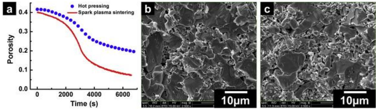
Fig. 2. (a) Porosity variation of ZrN powder densified (60 MPa and 10 °C/min) by SPS (1100 °C) and HP (1200 °C); images of the fractured surface of samples densified by (b) SPS at 1100 °C and (c) HP at 1200 °C.
