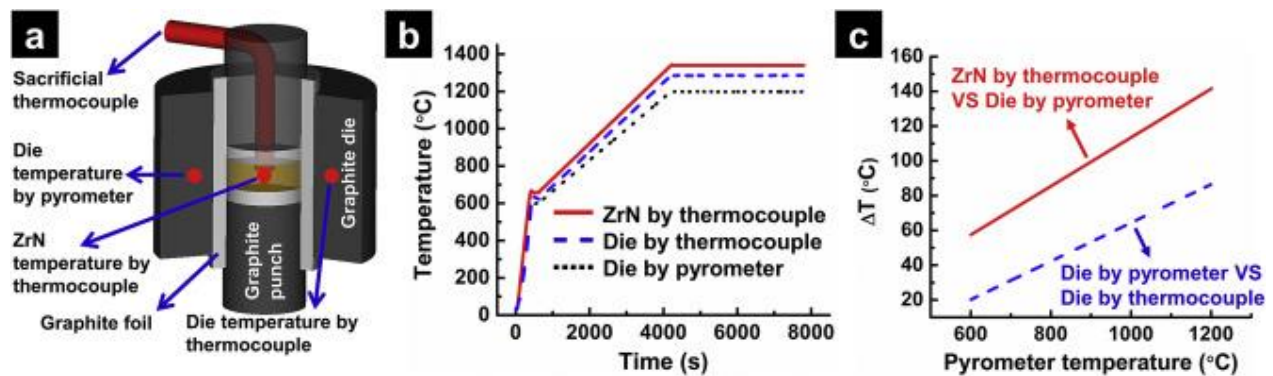
Fig. 1. (a) Schematics of SPS setup with temperature measurement points, (b) Temperature evolution of different measurement spots: SPS at 1200 °C under 60 MPa and 10 °C/min (red solid line: ZrN temperature by thermocouple, blue dash line: die temperature by thermocouple, black dot line: die temperature by pyrometer), (c) Differences ( \Delta T ) between ZrN temperature measured by thermocouple and die temperature measured by pyrometer (red solid line), and between die temperature measured by pyrometer and die temperature measured by thermocouple (blue dash line). (For interpretation of the references to colour in this figure legend, the reader is referred to the web version of this article.)
