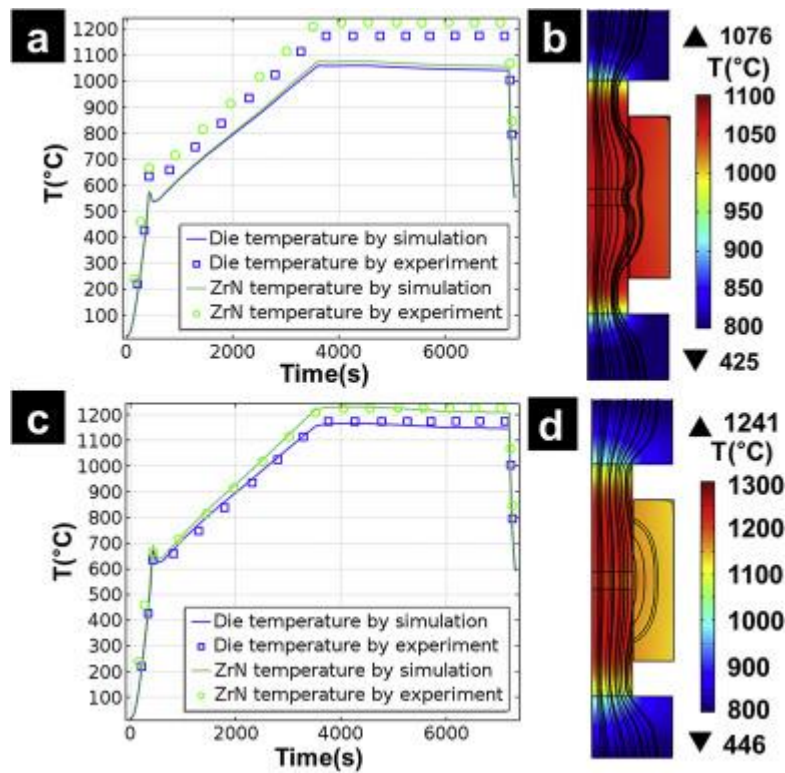
Fig. 3. Experimentally measured and FEM-simulated temperatures of ZrN powder and graphite die during SPS thermal cycle (a) without contact resistance, (c) with electrical and thermal contact resistance. FEM simulation map of the temperature and electric current flow at the end of the holding time (b) without contact resistance, (d) with electrical and thermal contact resistance. SPS at 1100 °C under 60 MPa and 10 °C/min was used.
