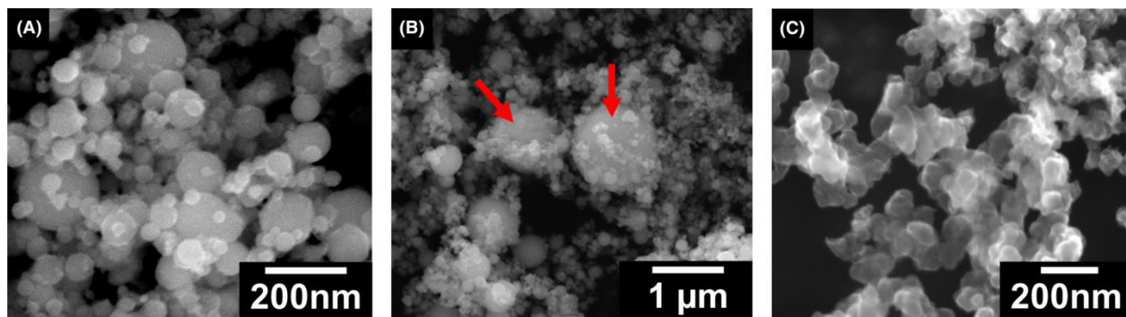
F2 SEM image A, 120 000× and B, 25 000× for Mo powders, and C, 100 000× for carbon powders. Red arrows indicate large Mo particles
