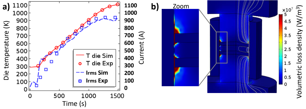
Figure 4: Compared experimental/simulated die temperature and electric current (a), simulated electric current lines and volumetric loss density (b).
