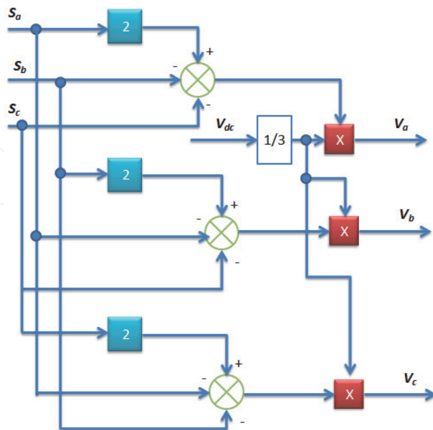
Figure 12. The block diagram of the RSC.
