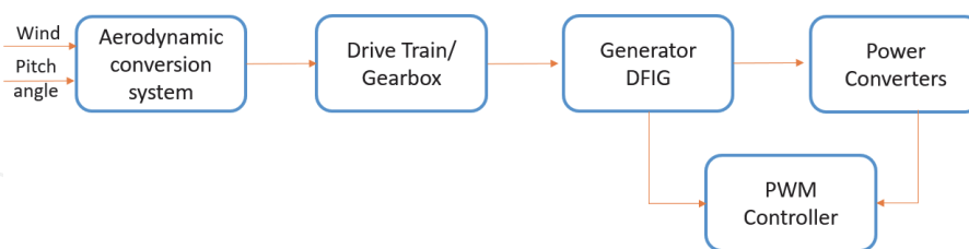
Figure 2. Wind turbine system structure.
