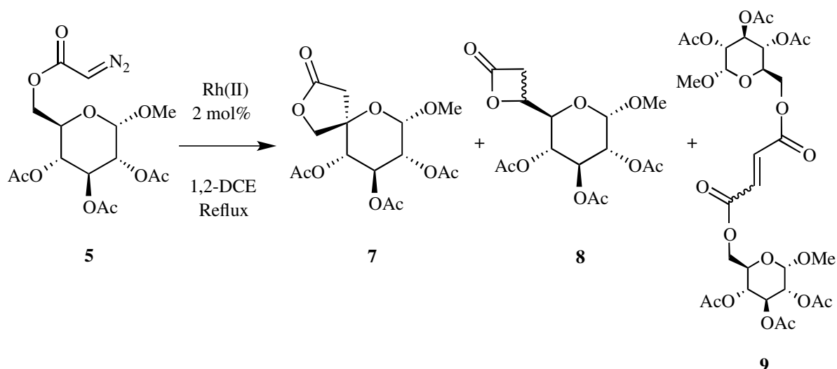
Scheme 3. Decomposition of 5 by \text{Rh}_2(\text{OAc})_4 .
