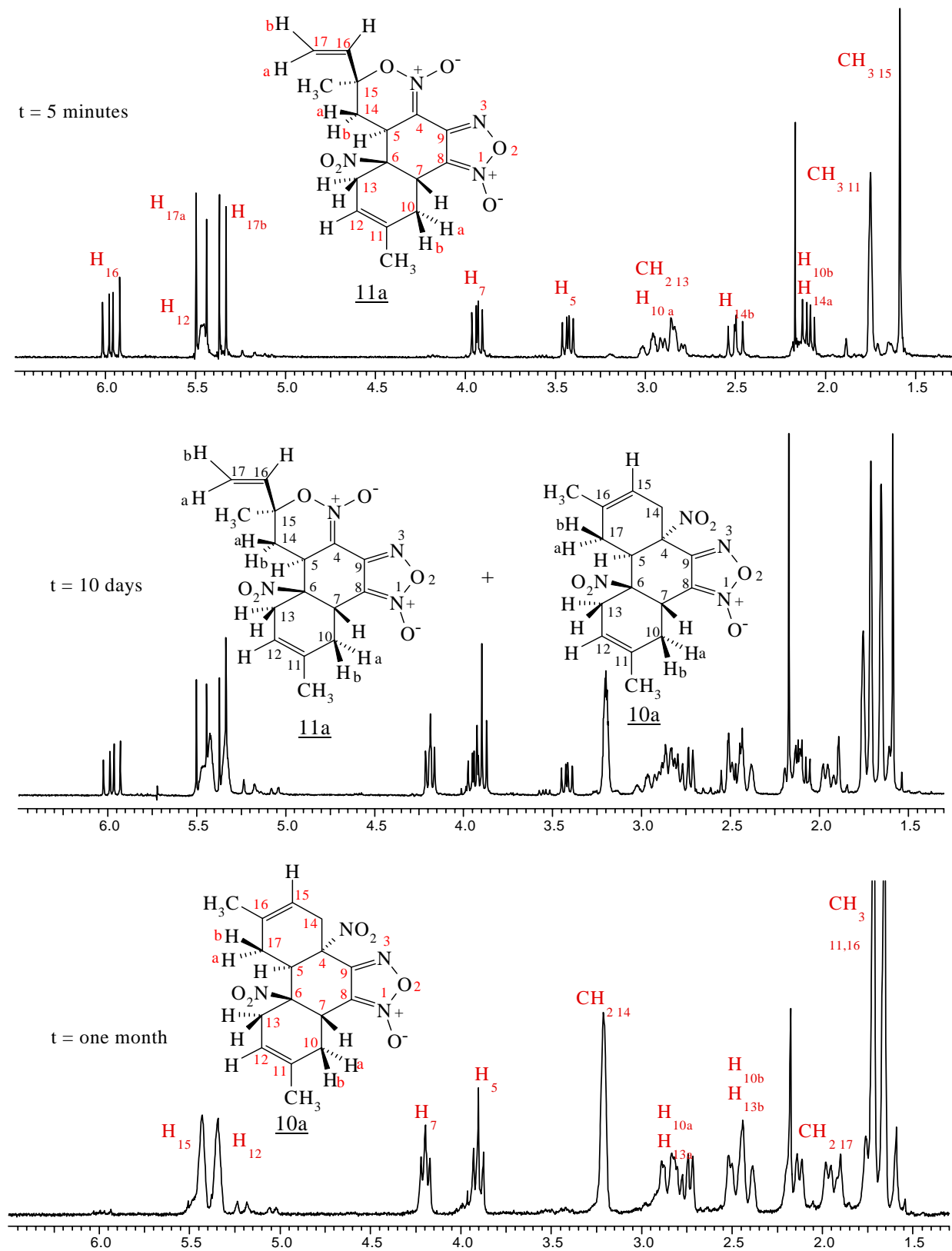
Figure 2. Time dependence of the ^1H NMR spectra of a pure sample of 11a in CDCl_3 .
