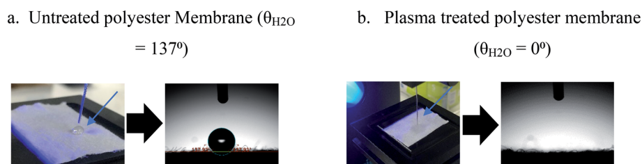
Fig. 3 Water contact angle analysis of (a) untreated and (b) plasma-treated polyester membrane using sessile droplet goniometry (digital image and fitting semicircle).
