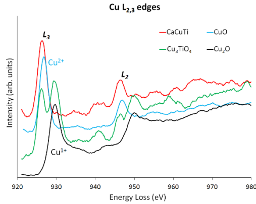
Fig. 15. Cu L_{2,3} edges ELNES spectra of \text{Cu}_2\text{O} , \text{Cu}_3\text{TiO}_4 , \text{CuO} and \text{CaCu}_3\text{Ti}_4\text{O}_{12} ( \text{CaCuTi} ), normalized to the peak height
