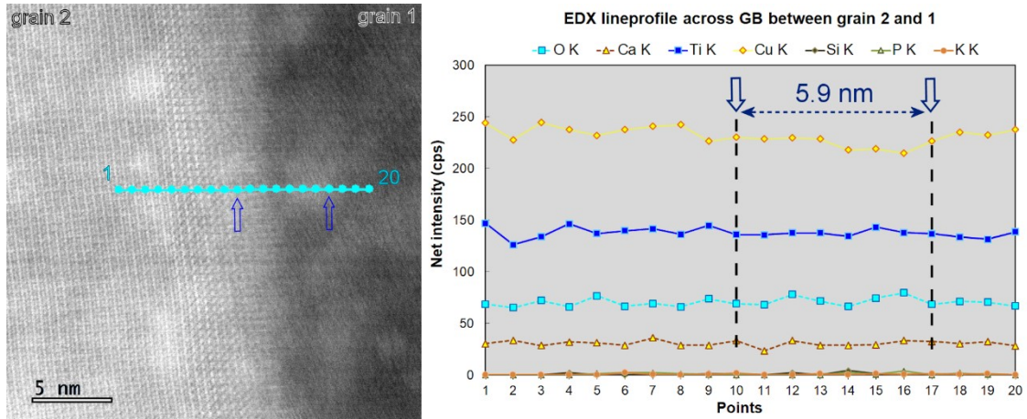
Fig. 6 HAADF-STEM image showing the location of the 20 points of EDX line profile across the GB; no significative variation of CuK line intensity is observed.
