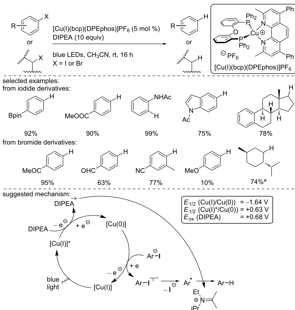
Scheme 20: Reduction of aryl and alkyl halides with the complex [\text{Cu}(\text{I})(\text{bcp})(\text{DPEphos})]\text{PF}_6 . a Irradiation was carried out at 420 nm. All redox potentials are reported vs SCE.
