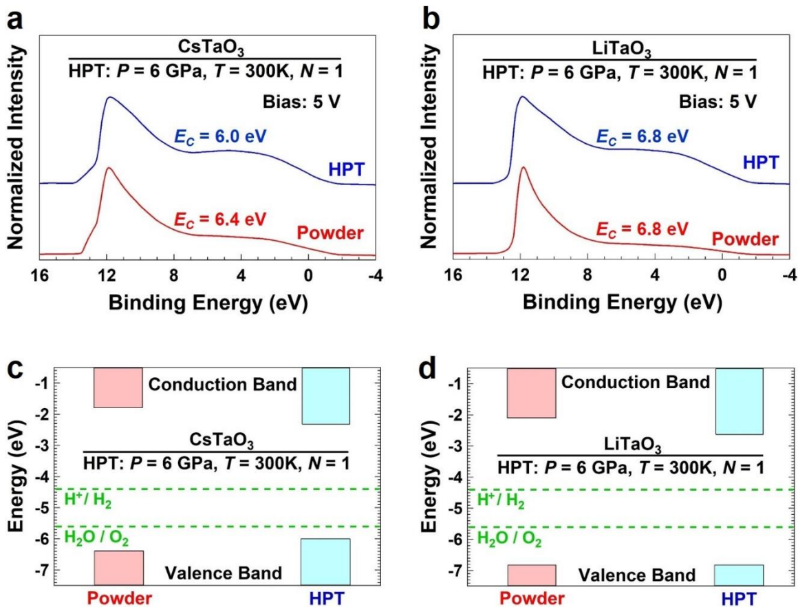
Figure 5. Changes in bandgap, valence band and conduction band energy levels in tantalate perovskites by severe straining. (a, b) UPS spectra and (c, d) band structure determined by UV-Vis reflectance spectroscopy and UPS for (a, c) \text{CsTaO}_3 and (b, d) \text{LiTaO}_3 before (powder) and after processing by HPT.
