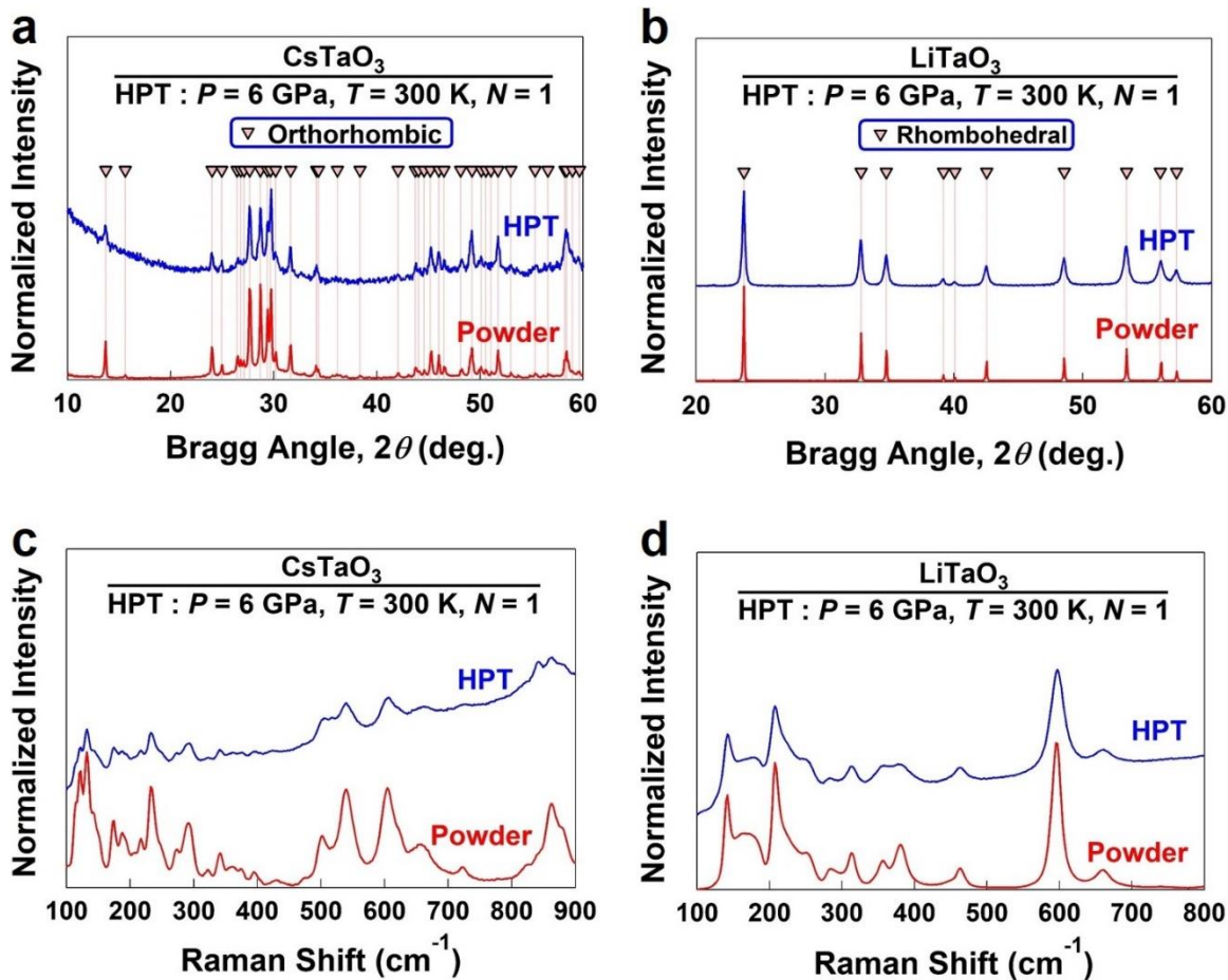
Figure 1. Formation of lattice defects without phase transformation to crystalline form in tantalate perovskites by severe straining. (a, b) XRD profiles and (c, d) Raman spectra for (a, c) CsTaO 3 and (b, d) LiTaO 3 before (powder) and after processing by HPT.
