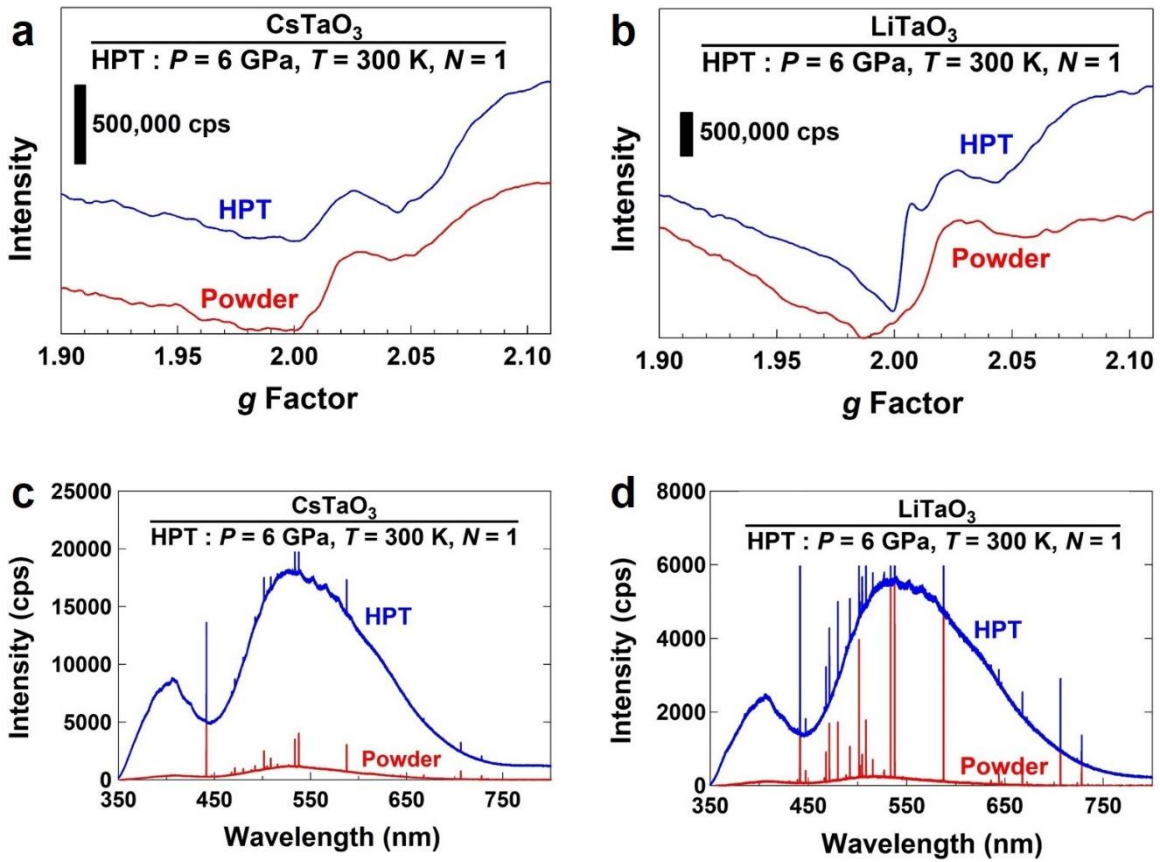
Figure 3. Formation of oxygen vacancies in tantalate perovskites by severe straining. (a, b) ESR spectra and (c, d) PL spectra for (a, c) CsTaO 3 and (b, d) LiTaO 3 before (powder) and after processing by HPT.
