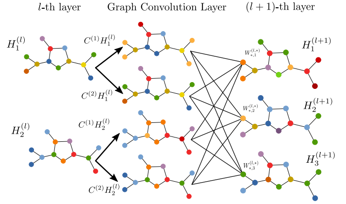
Fig. 1. Schematic of the GCN layer defined in (5). The graph has 12 nodes and 12 edges. Each node has a 2-length feature vector H_1^{(l)} and H_2^{(l)} represented by colors. The second layer has a 3-length feature vector, denoted H_1^{(l+1)} , H_2^{(l+1)} and H_3^{(l+1)} . Two convolution kernels C^{(1)} and C^{(2)} are used. This architecture has 12 trainable parameters, omitting biases.
