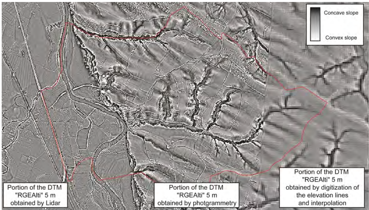
2 Fig. 12. Example of the problems related to the use of the DTM RGEAltI® 5 m resulting from a merging of elevation data from 3 several techniques and heterogeneous databases (location in red: municipality of Clermont-le-Fort, France). The map represents a 4 derivative (the curvature is represented by grey shades) from the same DTM obtained by merging different data sources (Bouroullec 5 et al., 2019)
