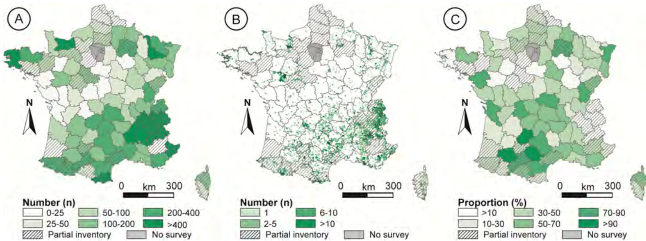
17 Fig. 11. BD-MVT and the systematic inventory status in France in 2019 (Source: http://www.georisques.gouv.fr/ ). A. Number of 18 inventoried landslides by department. B. Number of inventoried landslides by municipality. C. Proportion of landslides with 19 information about their size by department.
