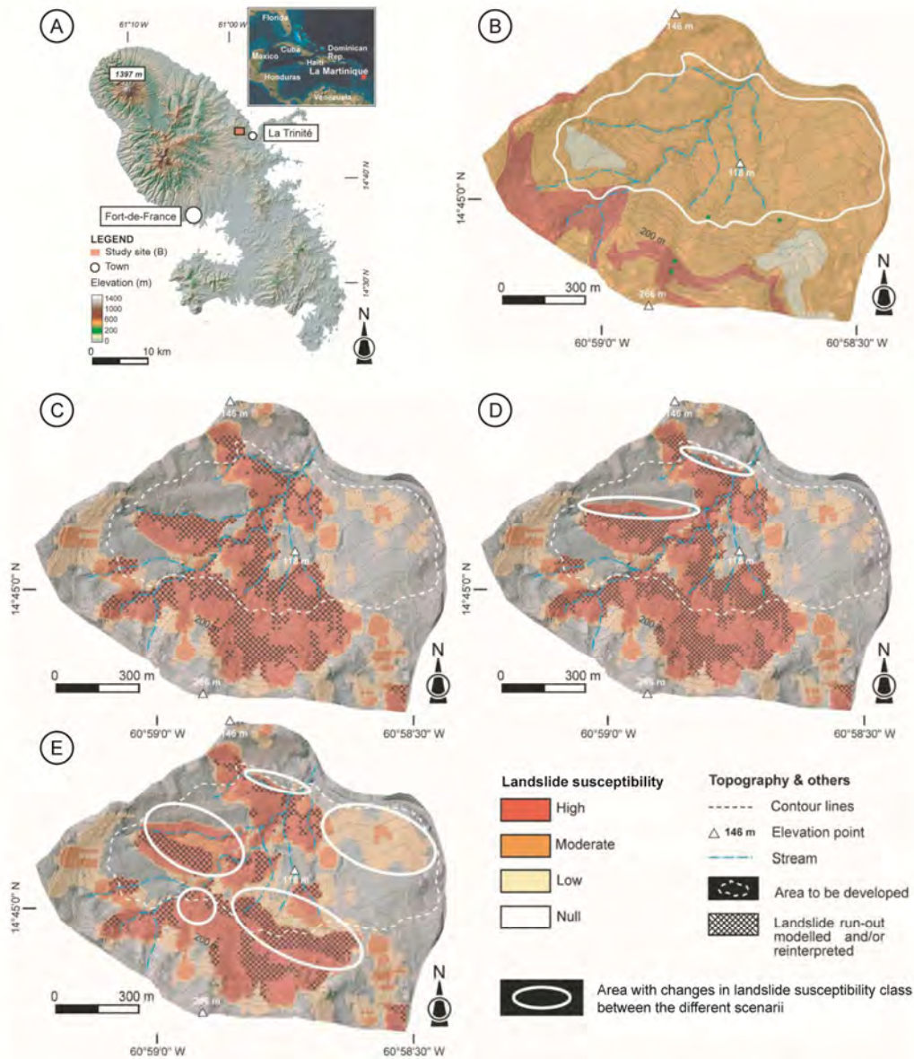
1 2 Fig. 13. Example of an ‘advanced’ susceptibility map for the community of La Trinité (Martinique, from Thiery et al., 2017b). A. 3 Location of the test site. B. Landslide susceptibility map produced by an empirical approach for the PPRN for the municipality of La 4 Trinité. C Advanced landslide susceptibility map produced by a physically-based model (ALICE®) for failure and a model based on 5 the angle of reach (BORA®) for the run-out of landslides; the map was produced for shallow and deep landslides. D. Advanced 6 landslide susceptibility map integrating expert knowledge on bank erosion and slope undercutting. E. Advanced landslide 7 susceptibility map integrating expert reasoning, bank erosion and slope works (excavations).
