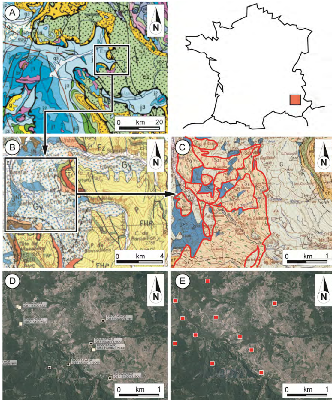
7 8 Fig. 10. Example of available information in the Infoterre webservice. This example is located near Embrun in the French South 9 Alps. A. Geological map at a 1:1,000,000 scale; the map shows the main lithology and structure for the area. B. Geological map at 10 a 1:250,000 scale; the map is more detailed, and it is possible to distinguish some surficial deposits interpreted by the geologist in 11 charge of the map. C. Geological map at a 1:50,000 scale; it is possible to obtain information on geomorphology, especially on the 12 slopes affected by landslides. D. Location of the main boreholes recorded in the BSS database and available in the Infoterre 13 webservice. E. location of the recent landslides recorded in the BD-Mvt database and available in the Infoterre webservice.
