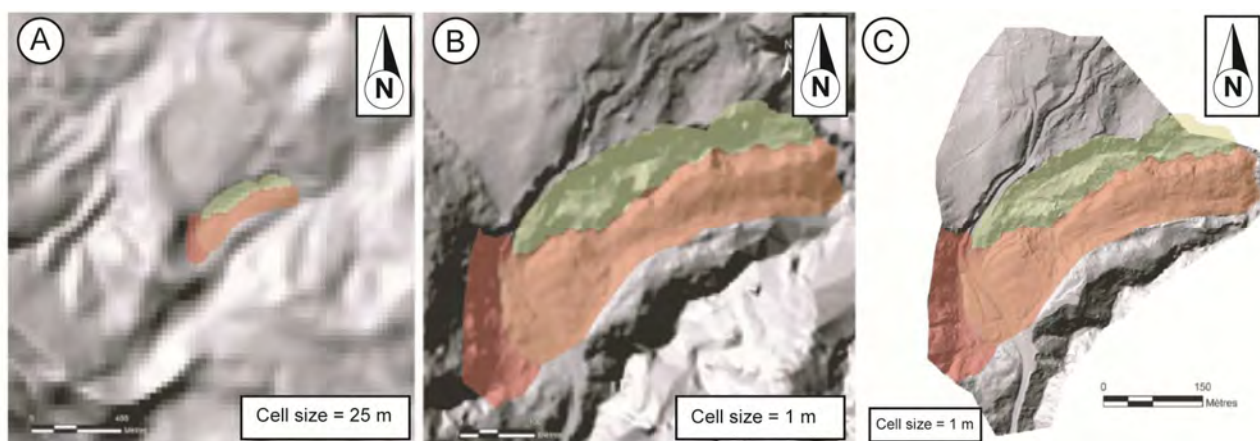
Fig. 6. Example of hillshade maps of the La Médaille landslide (La Martinique, France; Thiery et al., 2016). The DTMs were obtained at different resolutions and by different technologies. A. Hillshade map derived from BDAlti® with a resolution of 25 m. B. Hillshade map derived from Litto3D® (obtained by LiDAR, elevation resolution of 20 cm / planimetric resolution of 1 m). C. Hillshade map derived from a specific DTM obtained by LiDAR and created specifically for the site (elevation resolution of 10 cm / planimetric resolution of 20 cm – re-sampled to 1 m for the study).
