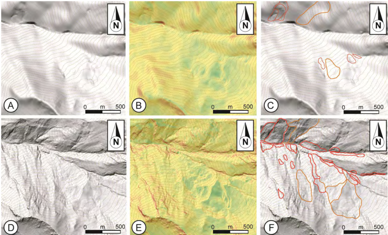
11 12 Fig. 7. Example of hillshade views and geomorphological interpretations for the Cauterets catchment (French Pyrenees, Thiery et 13 al., 2019b). A. Hillshade map derived from the DTM obtained by radar (cell size = 2 m). B. Slope map (cell size = 2 m) computed 14 from the DTM presented in A. C. Landslides inventoried from the analysis of A (red: active landslide; orange: inactive landslide). D. 15 Hillshade map derived from the DTM obtained by Lidar (elevation resolution 20 cm / planimetric resolution 20 cm; the cell size for 16 the figure is 2 m). E Slope map (cell size = 2 m) derived from the DTM presented in D. F. Landslides inventoried (red: active 17 landslide; orange: inactive landslide) from the analysis of D.
