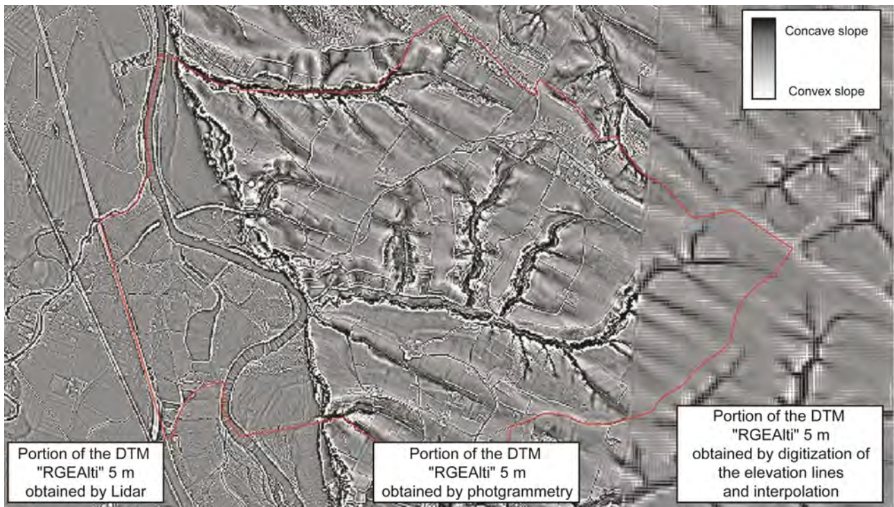
2 Fig. 12. Example of the problems related to the use of the DTM RGEAlt ® 5 m resulting from a merging of elevation data from 3 several techniques and heterogeneous databases (location in red: municipality of Clermont-le-Fort, France). The map represents a 4 derivative (the curvature is represented by grey shades) from the same DTM obtained by merging different data sources (Bouroullec 5 et al. , 2019)
