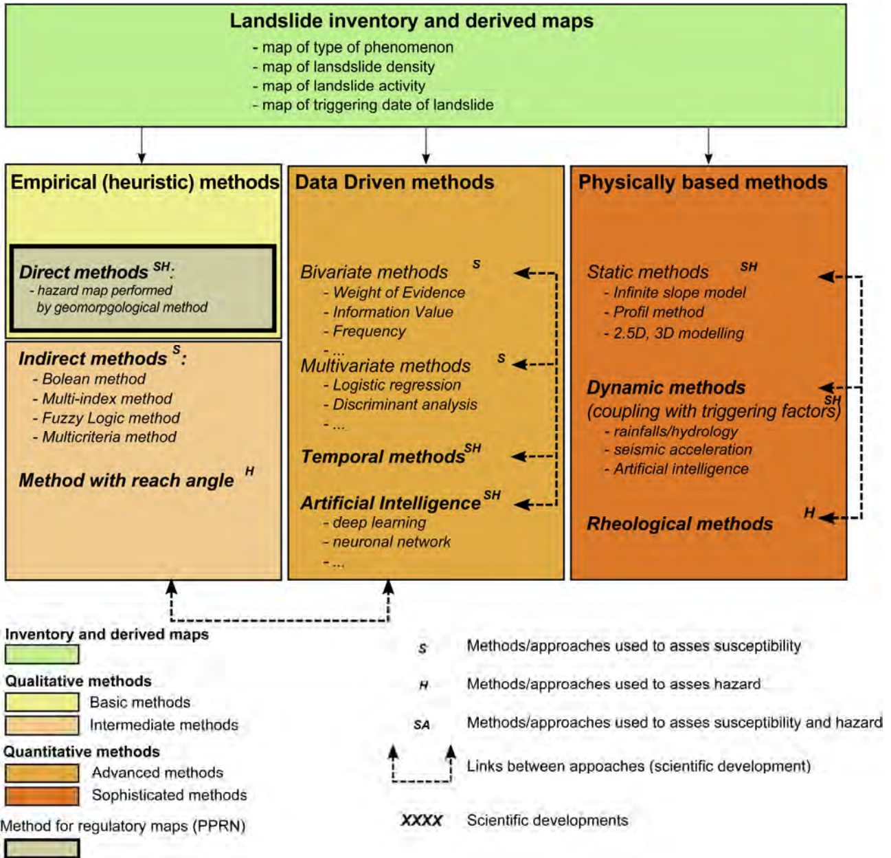
7 8 Fig. 4. Methods for landslide susceptibility and hazard assessment (from Soeters and van Westen, 1996; van Westen et al., 2006; 9 Fell et al., 2008; Corominas et al., 2014; Reichenbach et al. 2018).
