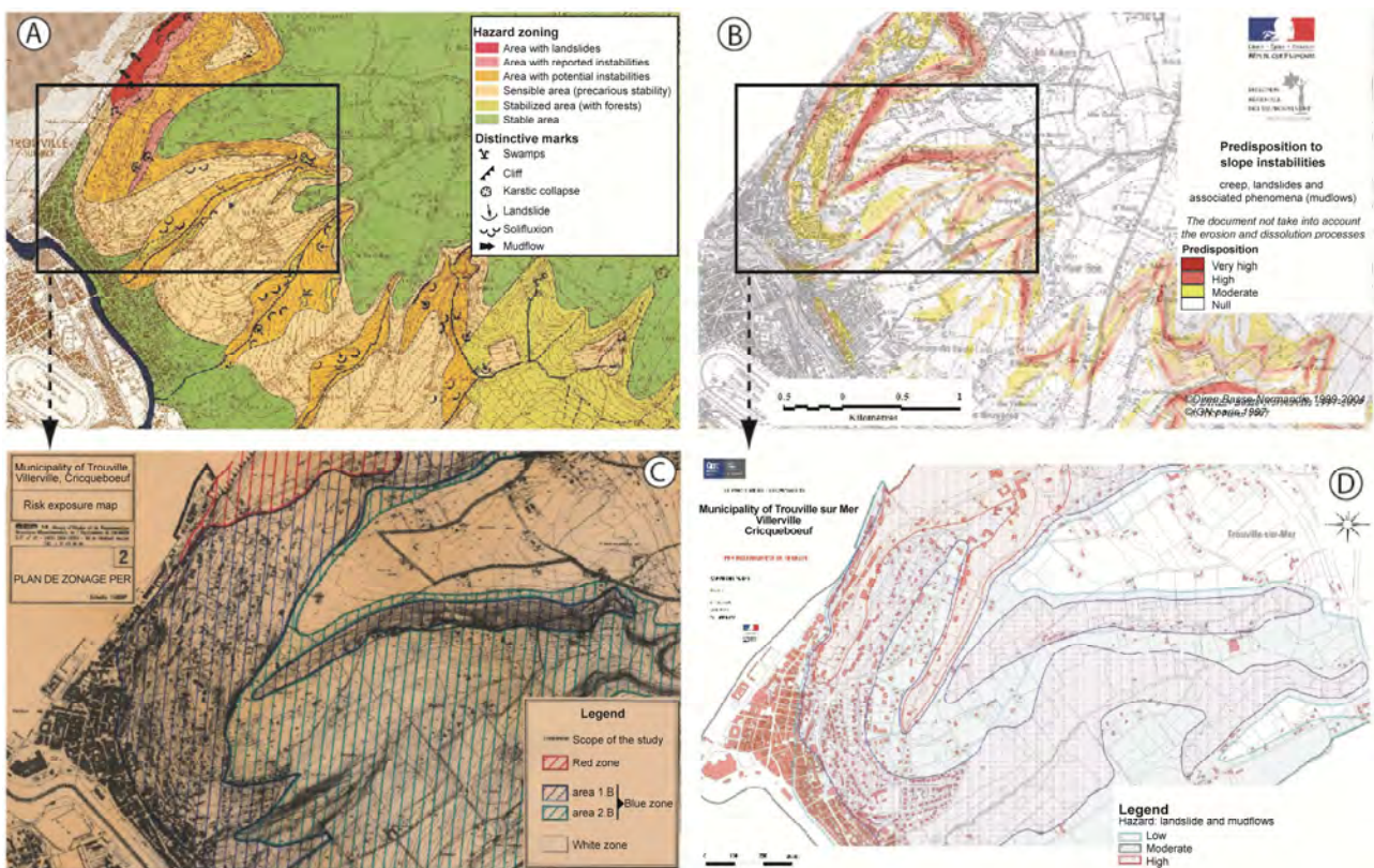
13 14 Fig. 2. Extracts of landslide hazard maps produced for different regulatory zoning. A. Extract of a ZERMOS hazard map for 15 Trouville/Pont l'Evêque at the 1:25,000 scale (BRGM, 1976). B. Extract from the landslide susceptibility map produced by a 16 combination of lithology and slope at the 1:25,000 scale (DREAL, 2004) C. Extract of the risk exposure map (PER) for 17 Trouville/Villerville-Cricqueboeuf at the 1:10,000 scale (LCPC, Rouen, 1986). D. Extract from the hazard map at 1:10,000 of the 18 Trouville/Villerville-Cricqueboeuf based on the PPRN procedure (DDTM, validated on 24 April 2009).
