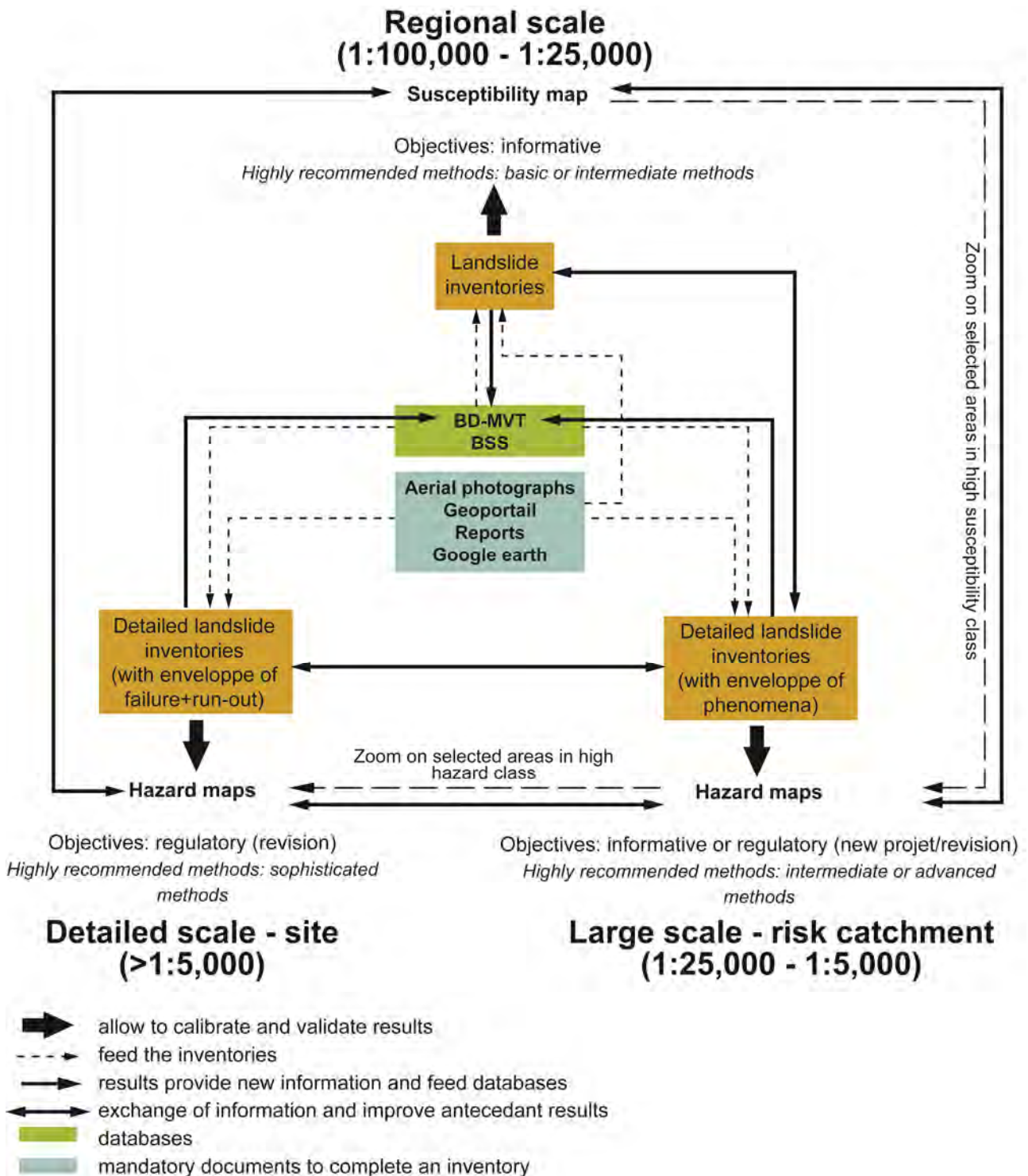
4 5 Fig. 14. Global landslide hazard assessment by a hierarchical strategy (nesting scale approach adapted from Leroi, 1996)
