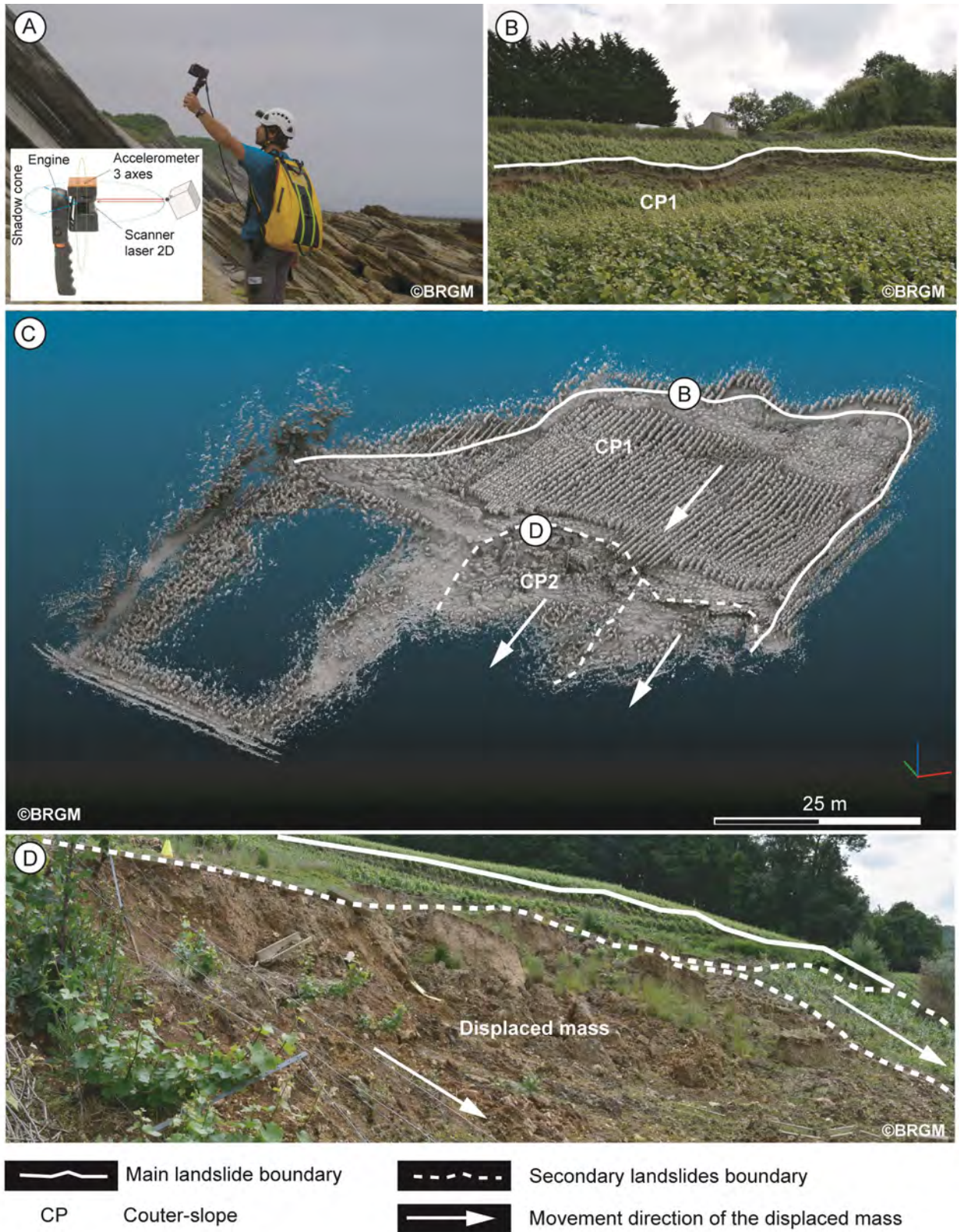
2 Fig. 5. Example of a point cloud obtained with a ZEB-Revo (a light, rotating 3D terrestrial laser scan) for a rotational landslide in 3 the vineyards of Champagne (Commune of Le Mesnil-le Huttier-2018). A. ZEB-Revo principles (measurements on the Socoa cliffs, 4 Pyrénées Atlantique, France). B. View of a landslide scarp. C. Point cloud and interpretation. D. View of the second landslide 5 scarp.
