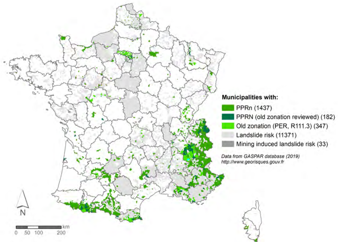
1 2 Fig. 1. Progress status for the landslide PPRN (landslide risk maps based on regulatory procedure) for 2019 e (source: 3 http://www.georisques.gouv.fr )
