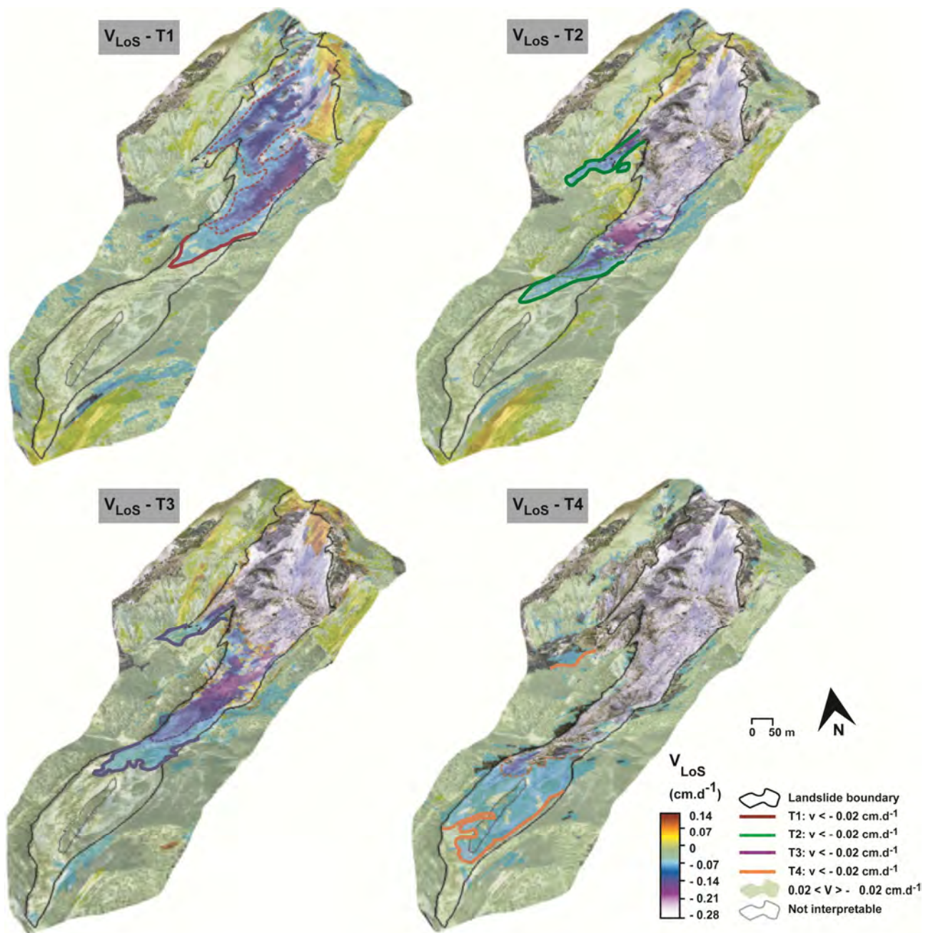
11 12 Fig. 8. Example of computed velocities based on ALOS/PALSAR image analysis for La Valette earthflow located in the 13 Barcelonnette basin, France (from Schlögel et al., 2015b).
