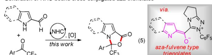
Scheme 1. Generation and reaction of various NHC-enolates.
