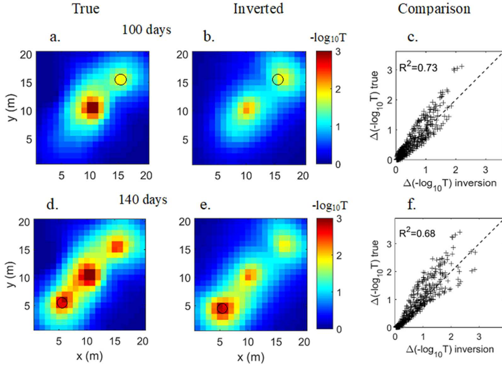
Figure 8: Changes in the hydraulic transmissivity over time. By column, from left to right: True field ( \Delta s_{true} ) - Inverted field ( \Delta s_{inv} ) - Comparison between them. By row, from top to bottom: t = 100, 140 days. The main decrease in the transmissivity field is located at the injection wells.
