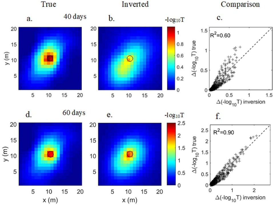
Figure 5: Changes in the hydraulic transmissivity induced by the particle injection at the center of the medium. By column, from left to right: True field ( \mathcal{A}_{true} ) - Inverted field ( \mathcal{A}_{inv} ) - Comparison between them. Inverted models outline the shape of the clogging area centered on the injection well.
