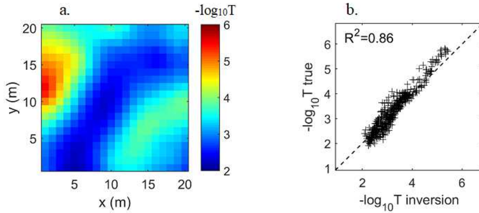
Figure 3: Estimation of the initial transmissivity field, which represents the hydraulic features of the aquifer before the injections: a) Inverted field, b) Comparison between the true and inverted transmissivity. The inverted field reproduce the major heterogeneity of the true transmissivity field and this initial inversion will serve as the starting point in the time lapse algorithm.
