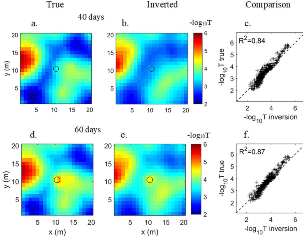
Figure 4: Injection occurs in the center of the medium (well # 5, black circle). By column, from left to right: True transmissivity field ( s_{true}^t ) - Inverted transmissivity field ( s_{inv}^t ) - correlation between them. By row, from top to bottom: T = 40 days, T = 60 days. The inverted results highlight the main variations in hydraulic transmissivity located around the injection well.
