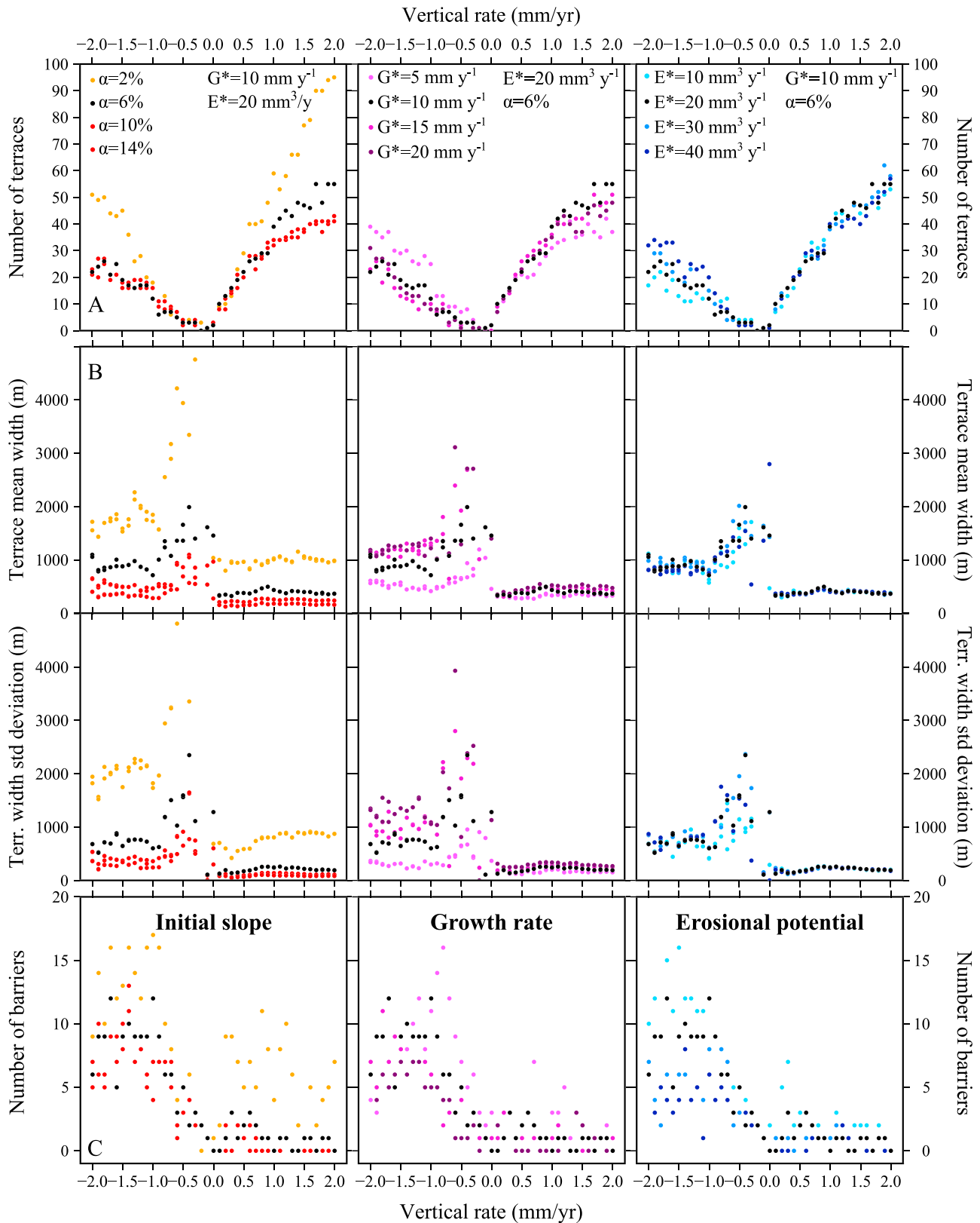
Figure 7. Systematics of modeled reefal sequences architectures, for variable sets of parameters with respect to reference values (black dots, G^* = 10 mm/year, \alpha = 6\% , E^* = 20 mm 3 /year; other parameters as in Table 1), varying slope \alpha (left column), potential reef growth G^* (middle column), and erosion potential E^* (right column). (a) Number of terraces in reefal sequences, (b) average width and standard deviation of the width of terraces, and (c) number of preserved modern and fossil barrier reefs.
