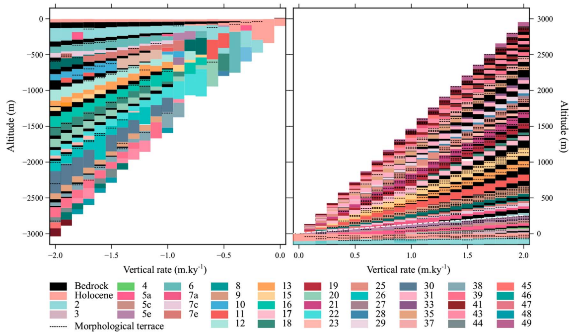
Figure 10. Modeled architectures—or kinematic barcodes —of subsiding (left) and uplifting (right) reefal sequences for a range of subsidence and uplift rates (from -2 to 0 mm/year, left; from 0 to 2 mm/year, right), as revealed by the last MIS of construction of terrace flats or fossil barriers prior to abandonment. Multiple terraces formed during a single cycle of eustatic variations are shown by dashed lines. All parameters but vertical rates are those of the reference case ( G^* = 10 mm/year, \alpha = 6\% , E^* = 20 mm/year; other parameters as in Table 1). Dashed white line indicates theoretical elevation of the highstand of MIS 5e according to Waelbroeck et al. (2002). MIS = Marine Isotopic Stage.
