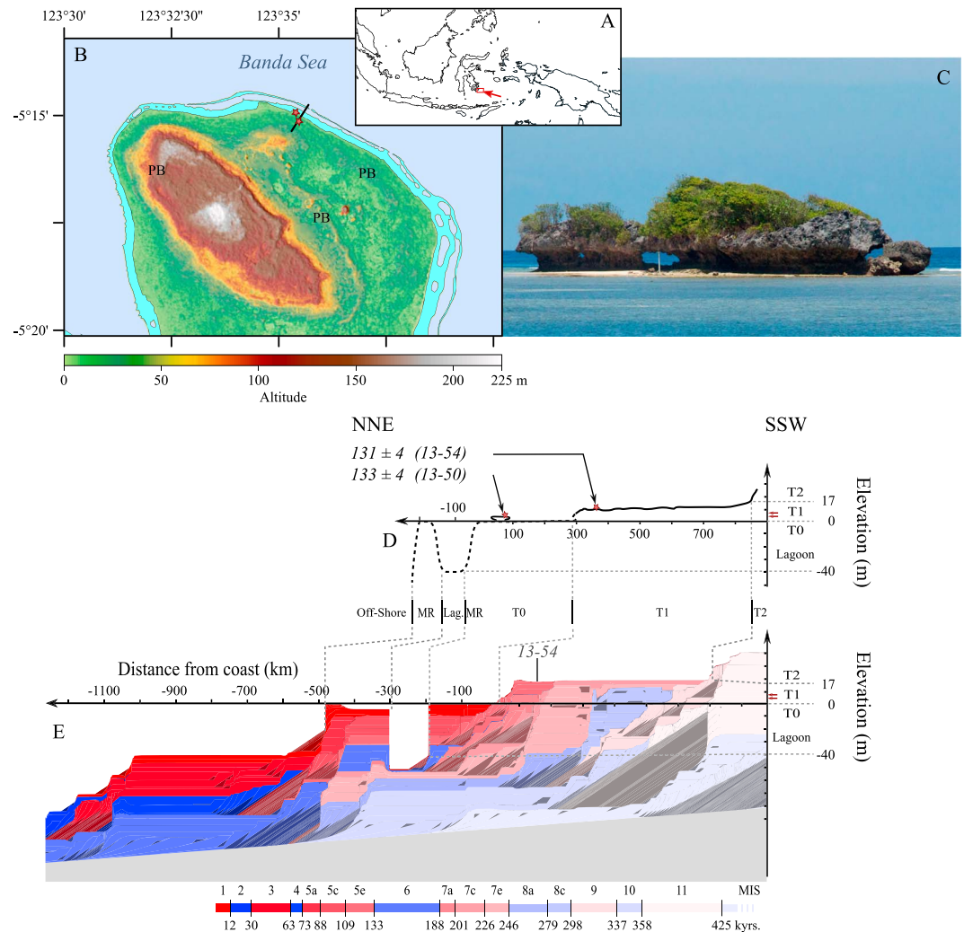
Figure 5. Wangi-Wangi island. (a) Location of the Tukang Besi archipelago, Indonesia. (b) Topographic map of northern Wangi-Wangi (SRTM30): light blue area shows modern reefs and platforms, PB = paleobarrriers, black line shows location of the detailed topographic profile, and red stars location of dated coral samples. (c) Emerged sea stack, relict of the fossil sequence, location of the northernmost sample, GSL-2013-50. (d) Synthetic topographic profile from differential Global Positioning System and sonar records, stars locate the dated samples. (e) Best fit simulation from the terrace model ( U = 0.1 mm/year, \alpha = 2\% , G^* = 15 mm/year, E^* = 30 mm 3 /year). Color scale as in Figure 4b.
