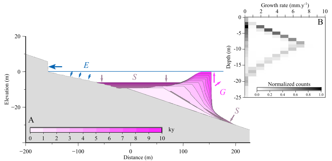
Figure 2. (a) Model output after a 10-kyr short simulation. Gray domain is the basement (initially having a linear surface), blue line is sea level, pink units are reef bodies, color-coded by age every 1 kyr. Shaded units are sedimentary layers. G , E , S , and U denote reef growth rate, erosion rate, sedimentation rate, and rate of vertical land motion, respectively. Parameters are as follows: stationary absolute sea level, G^* = 10 mm/year, U = -1 mm/year, E^* = 3 \cdot 10^{-2} m 3 /year, \alpha = 10\% . (b) Distribution of effective vertical reef accretion rate for several simulations over 1.5 Myr. U ranges from -2 to 2 mm/year, G^* = 10 mm/year, \alpha = 6\% , E^* = 20 mm/year.
