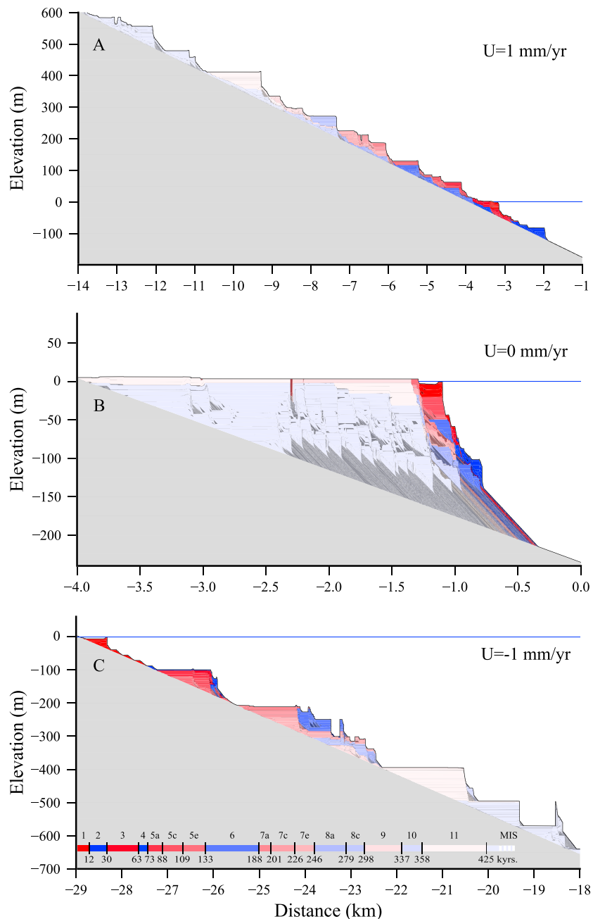
Figure 6. Simulations for three contrasted vertical rates: (a) fast uplift, 1 mm/year; (b) stationary, 0 mm/year; (c) fast subsidence, -1 mm/year (for reference values G^* = 10 mm/year, \alpha = 6\% , E^* = 20 mm/year; other parameters as in Table 1). Time evolution animations are provided online (supporting information).
