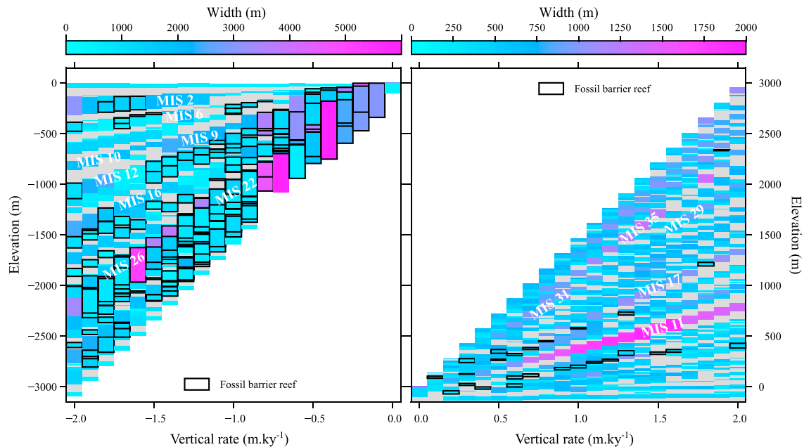
Figure 9. Modeled architectures—or morphological barcodes —of subsiding (left) and uplifting (right) sequences of coral reefs for a range of subsidence and uplift rates (from -2 to 0 mm/year, left; from 0 to 2 mm/year, right), as revealed by the morphology of the sequences. Terrace widths are color coded; their heights are given by the thickness of individual blocks. Solid black outlines indicate occurrences of fossil barriers. Gray areas represent the absence of any automatically detected terrace (bare foundations outcrop). Note the distinct color scales for subsidence (left) and uplift (right). All parameters but vertical rates are those of the reference case ( G^* = 10 mm/year, \alpha = 6\% , E^* = 20 mm/year; other parameters as in Table 1).
