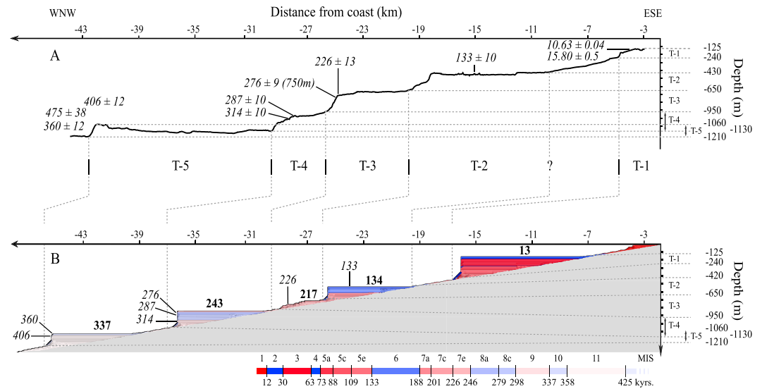
Figure 4. (a) Bathymetry of the NW Hawaii sequence (from MBARI Mapping Team, 2000). Dated samples (ages in ka are italicized) are either found along the profile or projected laterally (from Ludwig et al., 1991; Webster et al., 2007). (b) Modeled architecture of the reef sequence for the best fitting simulation, with equivalent locations for dated samples (italicized) and last age of construction for each terrace prior to abandonment (in bold). Color scale shows glacial (blue) and interglacial (red) isotopic stages; color saturation denotes age and increases with younger ages. Parameters: composite sea level curve concatenated from Waelbroeck et al. (2002) and Bintanja et al., 2005 (2005; see section 2.4), U = -3 mm/year, \alpha = 3\% , G^* = 7 mm/year, z_{\max} = 50 m, E^* = 5 \cdot 10^{-2} m 3 /year.
