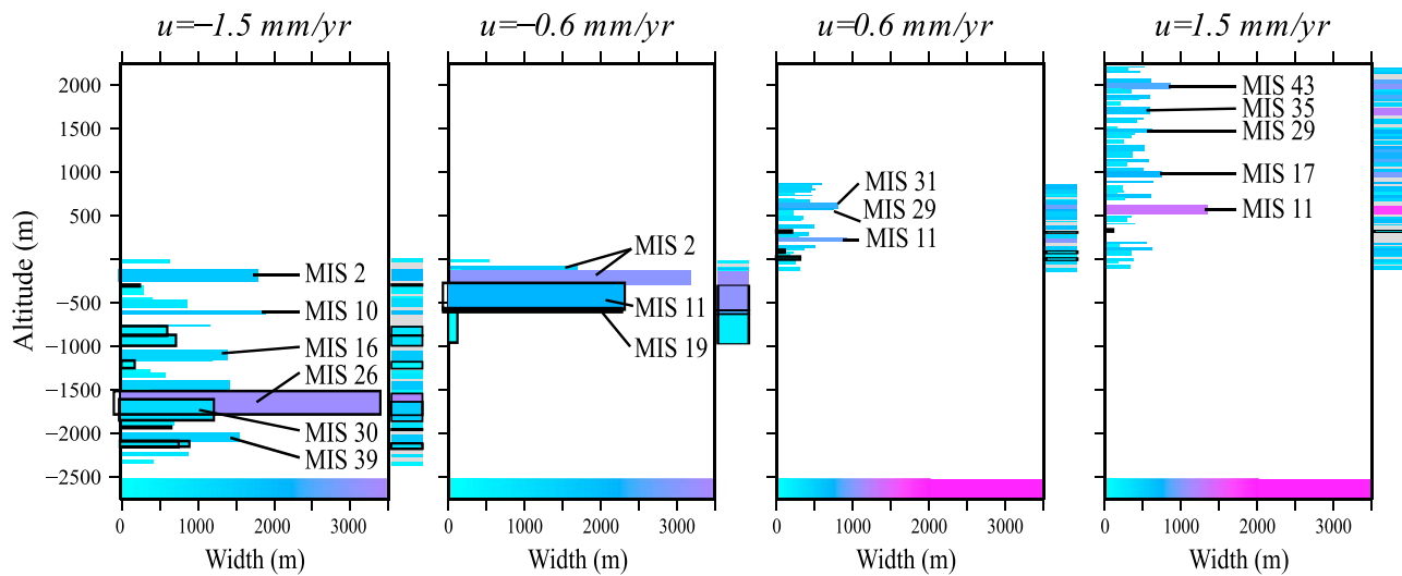
Figure 8. Modeled architectures—or barcodes —of two subsiding sequences (first and second panels, -1.5 and -0.6 mm/year) and two uplifting sequences (third and fourth panels, 0.6 and 1.5 mm/year). The morphology of the sequences is summarized by the relative distribution of terraces, each of them being defined by their widths (as they appear in abscissae) and heights (as revealed by the thickness of individual segments) and by the occurrence of fossil barriers (solid black outlines). The isotopic stage corresponding the last episode of reef construction on the terrace flat or barrier is indicated for prominent features. The external architecture of each sequence is synthesized into barcodes, with similar color scales for terrace width, on the right of each graph.
