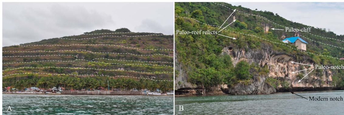
Figure 1. (a) Sequences of emerged reef terraces, Sampolawa Bay, SE Sulawesi (Fortuin et al., 1990; Padoja et al., 2018). White dashed lines delineate uplifted terraces. (b) Close-up showing nested narrow terraces and fossil notches. The active notch is carving a retrograding cliff in earlier reefal units, which progressively erases earlier sea level markers. The erratic block in the forefront witnesses this retrogradation, while the preservation of fossil notches attests for moderate marine erosion.
