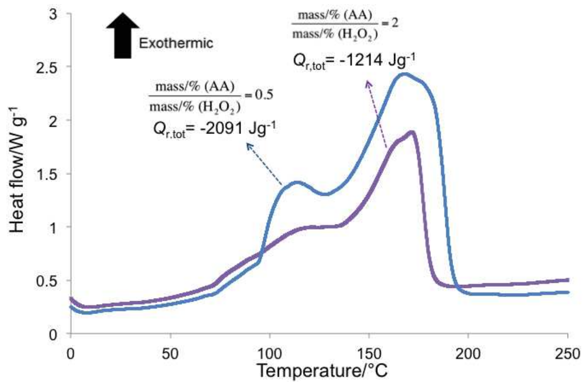
Fig. 3 DSC experiment at 4^{\circ}\text{C}/\text{min} at different ratio of acetic acid on hydrogen peroxide
