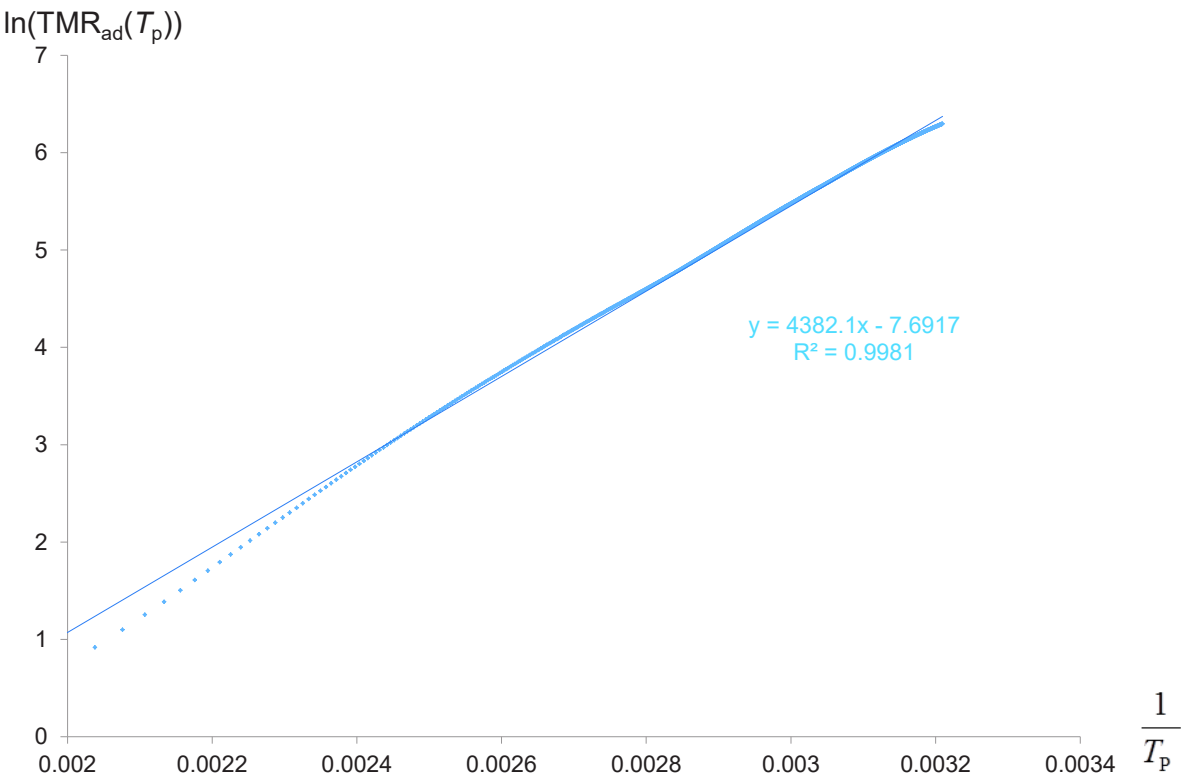
Fig.11 \ln(\text{TMR}_{\text{ad}}) versus T_p^{-1} / \text{K}^{-1}
