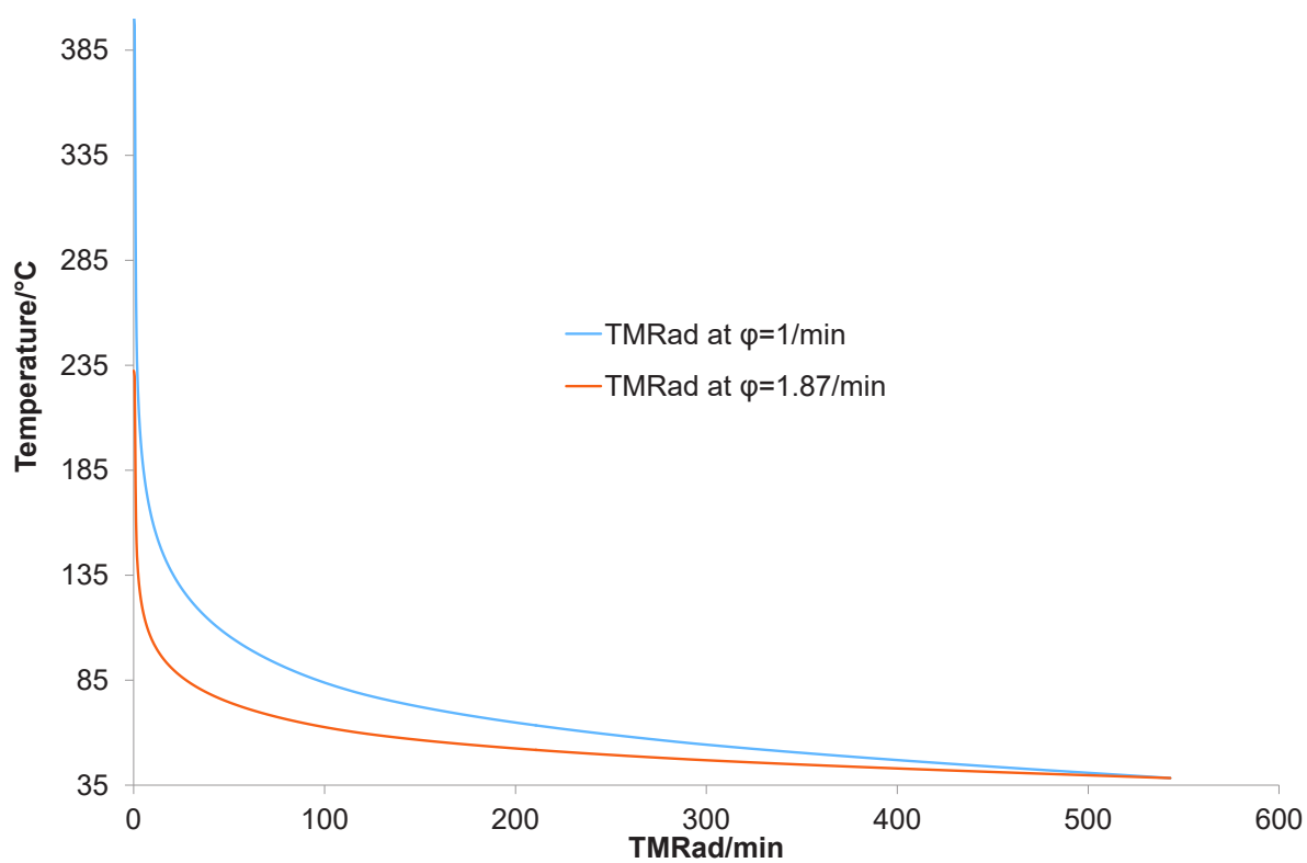
Fig. 10 Evolution of \text{TMR}_{\text{ad}} with \phi -factor
