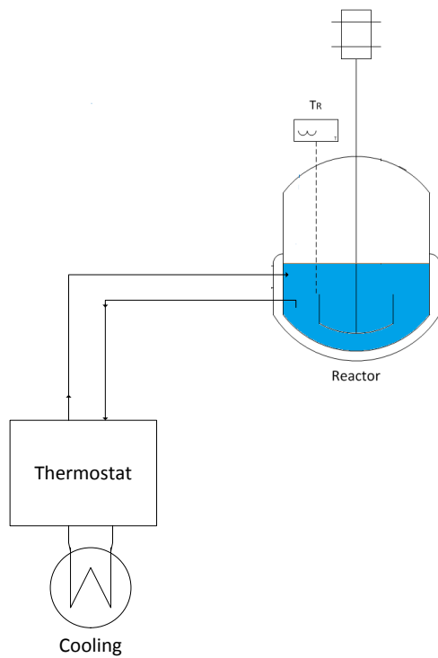
Fig. 21. Reactor system.
