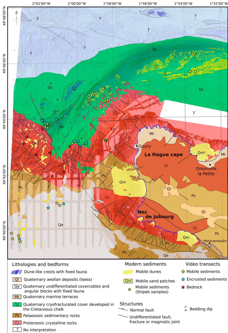
Figure 7. Non-exhaustive geological-sedimentary-dynamic map. The BRGM geological map is used for the onshore part and interpretations from our videos, Shipek samples and bathymetric map for the offshore part. The samples points are added and are colored according the dynamic dominance (mobile or sediments covered by fixed fauna).
