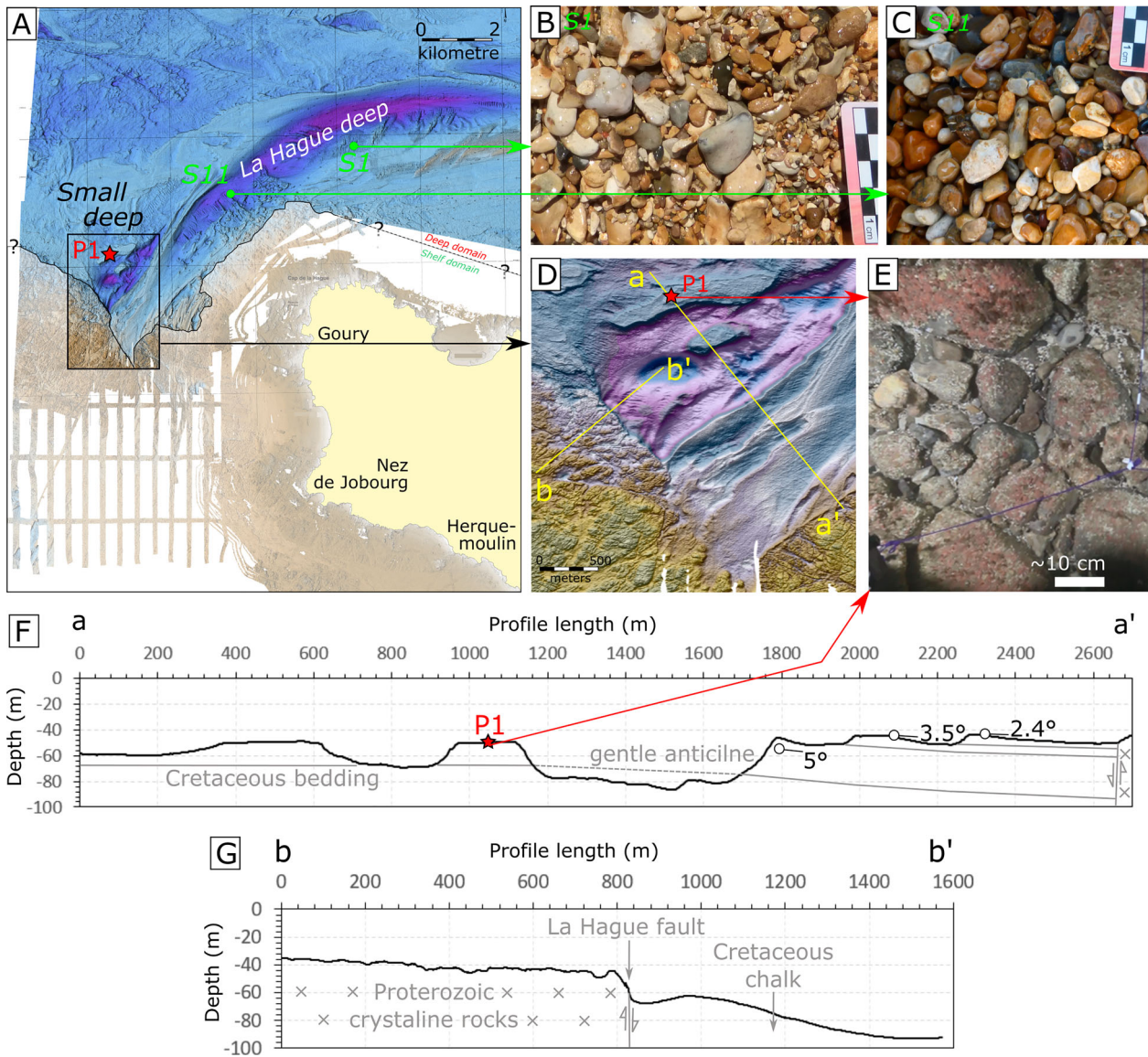
Figure 3. Bathymetry, samples and geologic interpretations of the La Hague deep and the small deep. (A). Bathymetric map of the Alderney Race showing the location of the La Hague deep and of the small deep; (B and C). Photographs of Shipek grab samples with cretaceous flint rocks pebbles collected in the La Hague deep. (D). Detailed bathymetric view of the small deep. (E). Photographs extracted with the underwater camera showing relatively angular cobbles and blocks with fixed fauna. (F and G). aa' and bb' transects with simple geologic interpretations.
