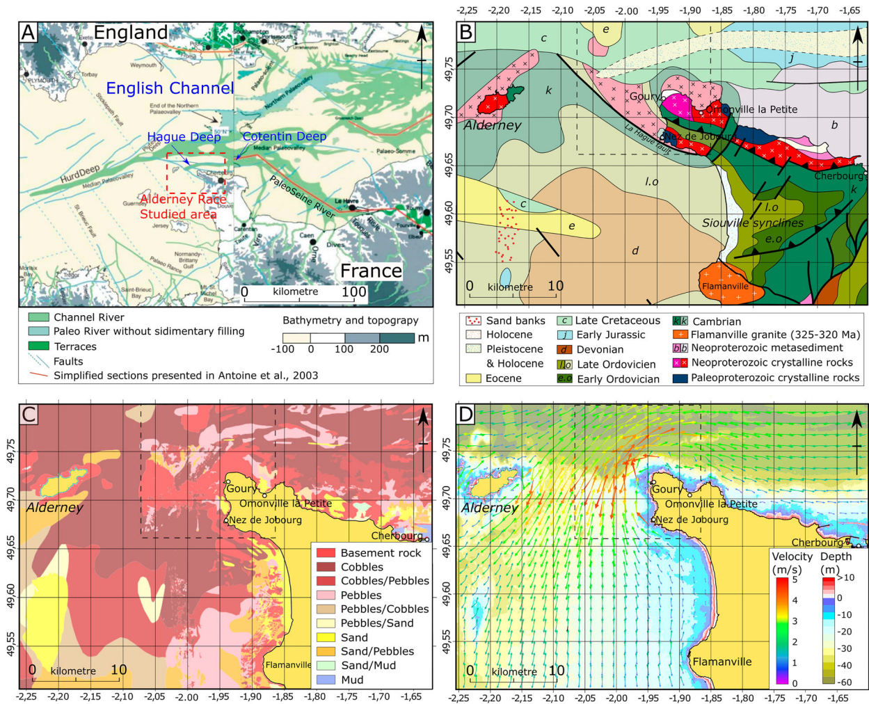
Figure 1. (A). Map of the English Channel showing the deeps that coincide with the paleo-Seine and its tributaries (Antoine et al., 2003) and the location of our study area (red rectangle); (B). Geological map (modified from geological map of France 1/50 000); (C). Sedimentary map (modified from data.shom); (D). Simplified bathymetric map showing the maximal tidal current intensities at high and low tides from numerical model MARS2D, resolution of 100 m (method from Bailly du Bois et al., 2012).
