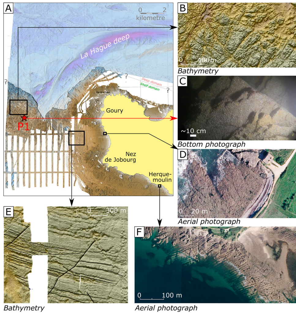
Figure 4. Examples of the bedrock morphologies in the shallow platform. (A). Bathymetric map of the Alderney Race showing the location of the detailed views of the bedrock (B and E), aerial photographs (D and F) and submarine photograph (C). Crystalline Proterozoic (B) and sedimentary Paleozoic (E) bathymetric morphologies compared to their coastal equivalents from aerial photographs from the Baie d’Ecalgrain (D) and Herquemoulin rocky platform (F).
