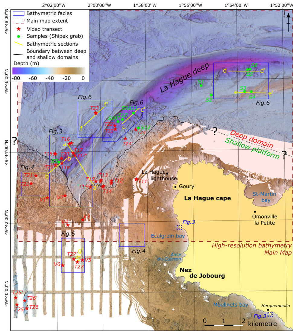
Figure 2. Bathymetric map of the Alderney Race with the location of video transects (red stars, named Tn or Vn with indicating the end of transect). Specific bathymetric morphologies (blue rectangles) are described in detail on the next figures. The yellow transects indicate the bathymetric sections. The dashed brown rectangle represents the high bathymetric map extent.
