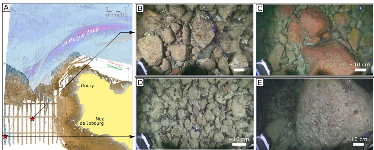
Figure 5. Examples of cobbles and blocks with fixed fauna and possible corestones in the shallow platform. (A). Bathymetric map of the Alderney Race showing the location of the submarine photographs. (B and D). submarine photographs showing cobbles with fixed fauna. (C and E). submarine photographs showing possible corestones.
