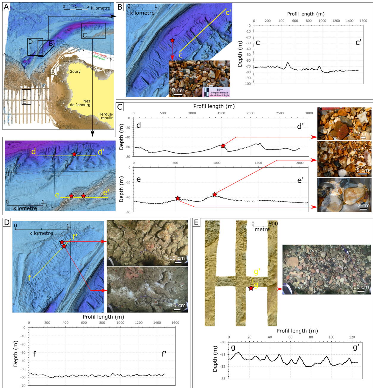
Figure 6. Examples of giant to very large dunes field in the Alderney Race. (A). Bathymetric map of the Alderney Race showing the location of the dune fields presented in this figure. (B and C). Detailed bathymetric map, longitudinal transects and Shipek grab samples of active dunes fields in the La Hague deep. (D). Detailed bathymetric map, longitudinal transect and submarine photographs of inactive dunes fields west of the La Hague deep. (E). Detailed bathymetric map, longitudinal transect and submarine photographs of active dunes fields in the shallow platform.
