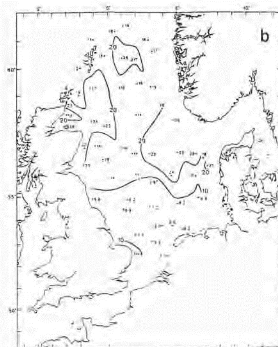
Fig. 13. Evaluation of the degree of renewal for waters in the North Sea between 1986 and 1988: (a) residual ^{134}\text{Cs} contribution during July 1988 due to direct fallout from the Chernobyl accident, (b) seawater ^{134}\text{Cs} activity in \text{Bq.m}^{-3} during August-September 1986 (alter MITCHELL & STEELE, 1988), and (c) estimate of degree of renewal (in %) for waters in the North Sea between July 1986 and July 1988.
