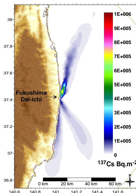
Fig. 1 Calculated cumulate deposit of ^{137}\text{Cs} , 2011 April 23
