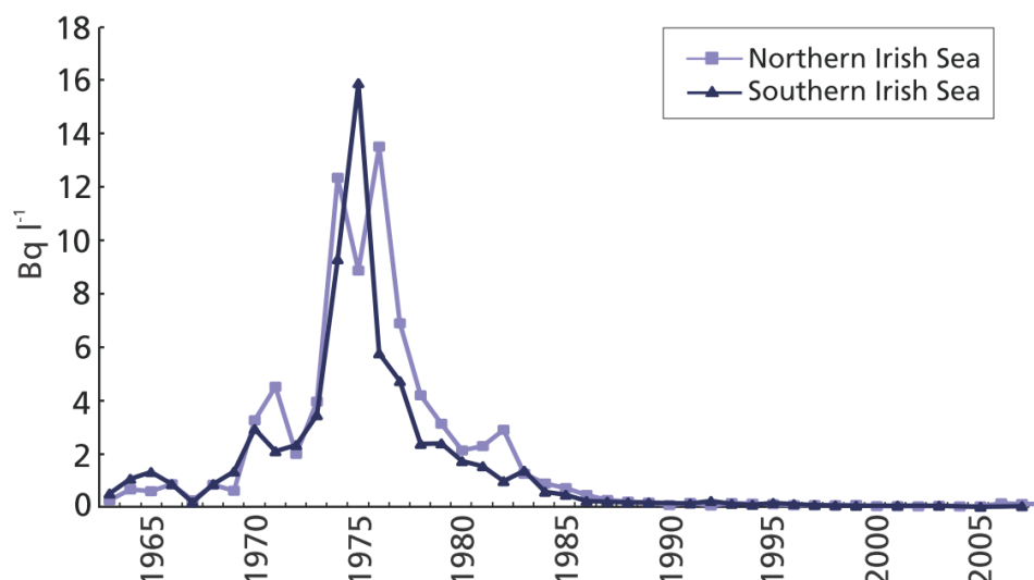
Fig. 7 Concentrations of 137 Cs in the Irish Sea seawater (from Rife, 2009)
