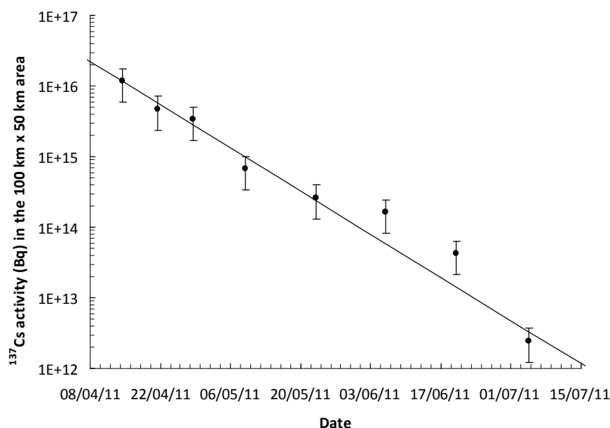
Fig. 5 Evolution of the 137 Cs quantities present in seawater at more than 5km from the coast.
