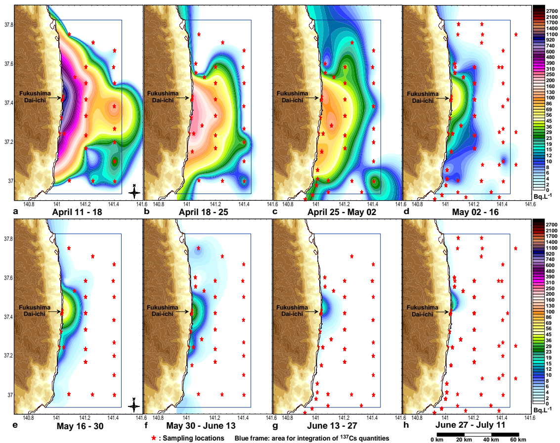
Fig. 4 Concentrations of ^{137}\text{Cs} in seawater between April 11 and July 11 2011.
