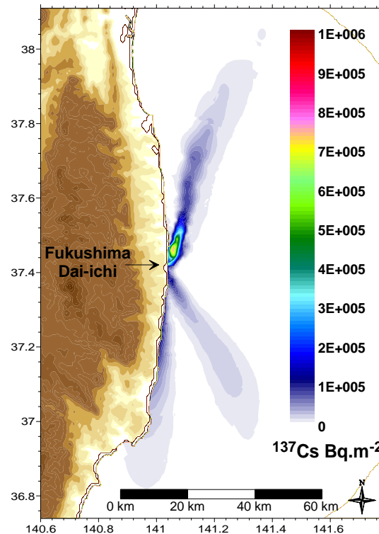
Fig. 1 Calculated cumulate deposit of 137 Cs, 2011 April 23
