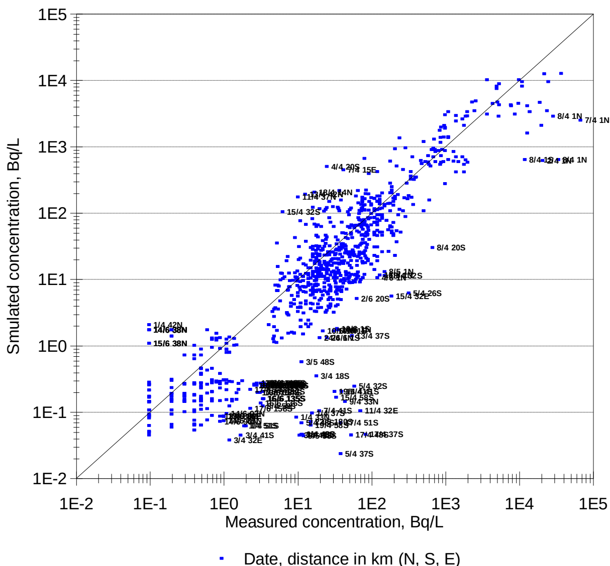
Figure 12. Measured versus simulated concentrations of ^{137}\text{Cs} for samples available between 1 April and 30 June. Dates and distances are reported when ratio is higher than 10.
