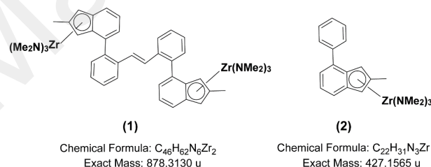
Scheme 1. Structures of dinuclear E-(o)-{BisInd}(Zr(NMe 2 ) 3 ) 2 isomer (1) and mononuclear {Ind}Zr(NMe 2 ) 3 (2) zirconium complexes used in this study.
