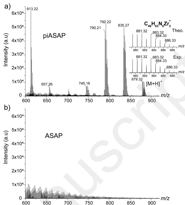
Figure 2. Analysis of E -Zr dimer ( 1 ) by piASAP and ASAP techniques. (a) and (b) are mass spectra of piASAP and ASAP conducted under inert and aerobic conditions, respectively. The zoomed areas showcase the theoretical and experimental isotopic patterns of complex 1 .
