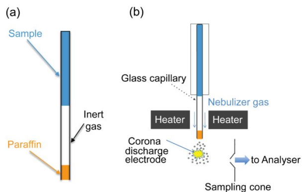
Figure 1. (a) paraffin-inert ASAP glass capillary. (b) paraffin-inert atmospheric solid analysis probe (piASAP) principle.
