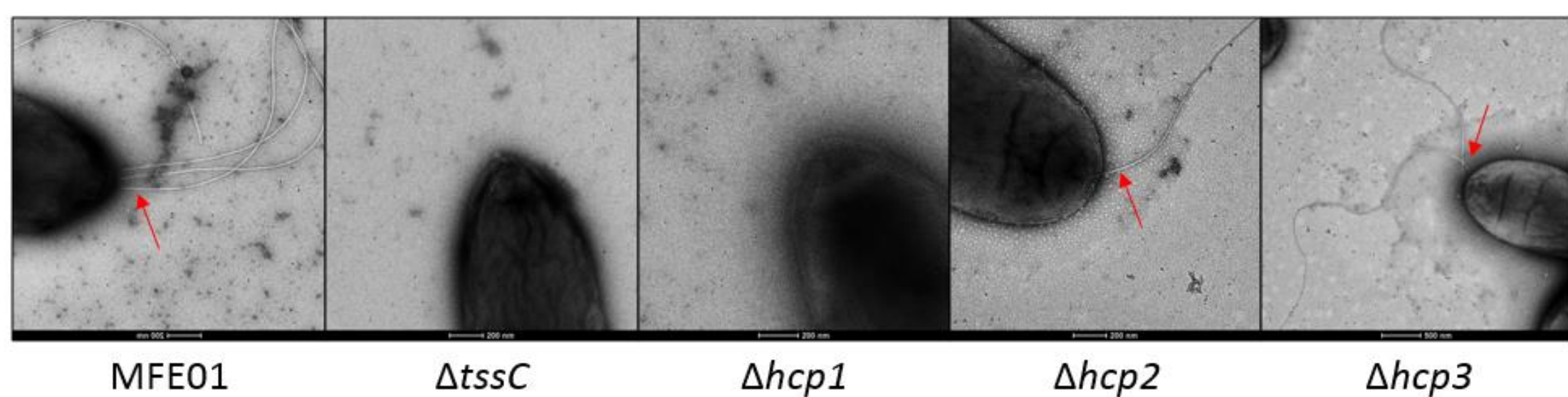
Figure n°3 : Electronic microscopy of MFE01 and different T6SS deletion mutants. Red arrows show flagellar filament (Gallique et al. , in progress).
