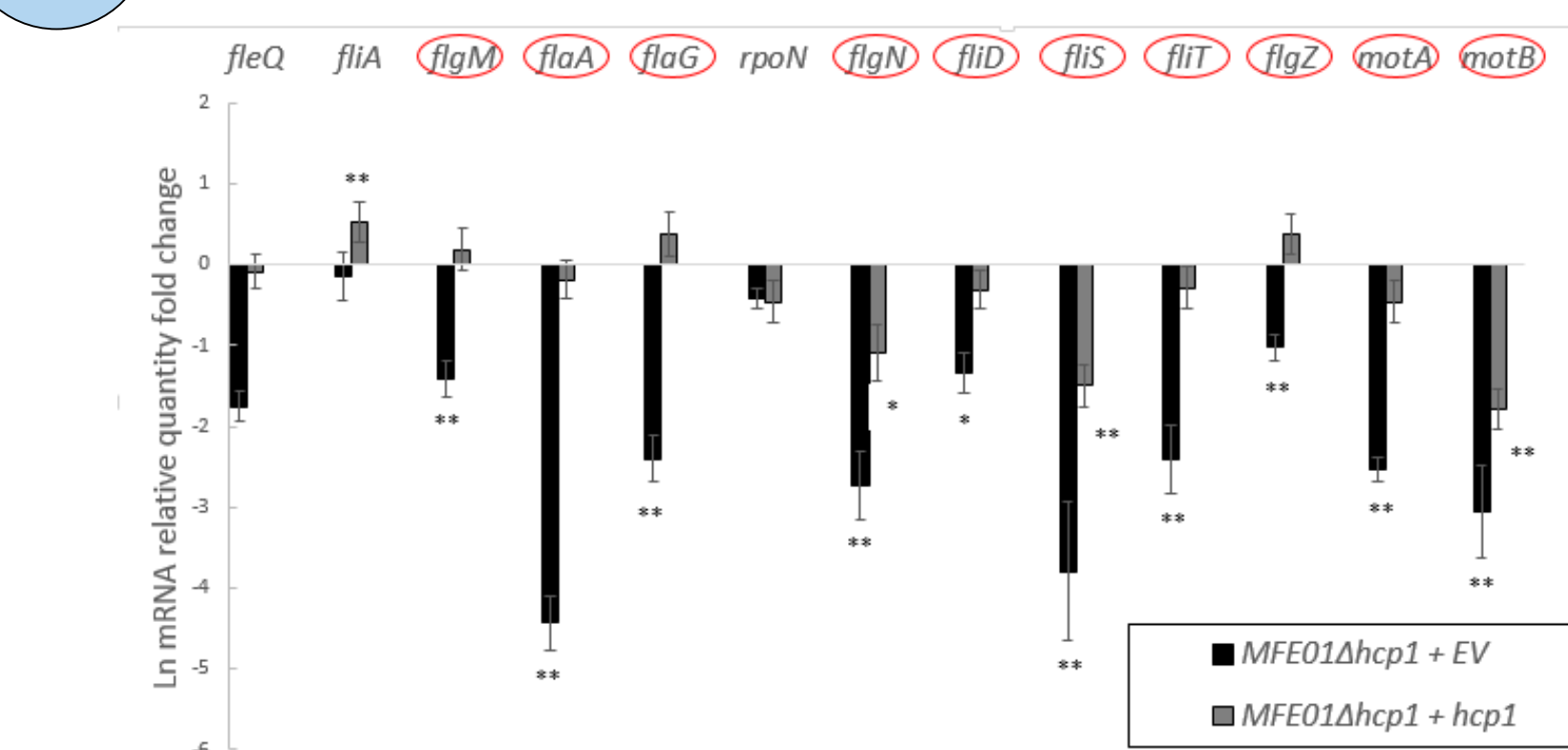
Figure n°4 : Expression of flagellar genes in MFE01 \Delta hcp1 +EV/+ hcp1 compared to wild type strain containing empty vector (EV). Data shown represent the mean \pm SEM. Significances of differences between mean values were assessed using Mann-Whitney test (n=6) with significance set as *P<0.05; **P<0,005. Red circles represent genes that are expressed by FliA sigma factor. (Gallique et al. , in progress).
