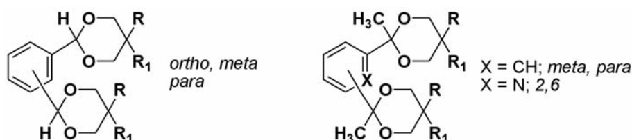
Scheme 1 General formulae of the investigated bis(1,3-dioxan-2-yl)arene derivatives.
