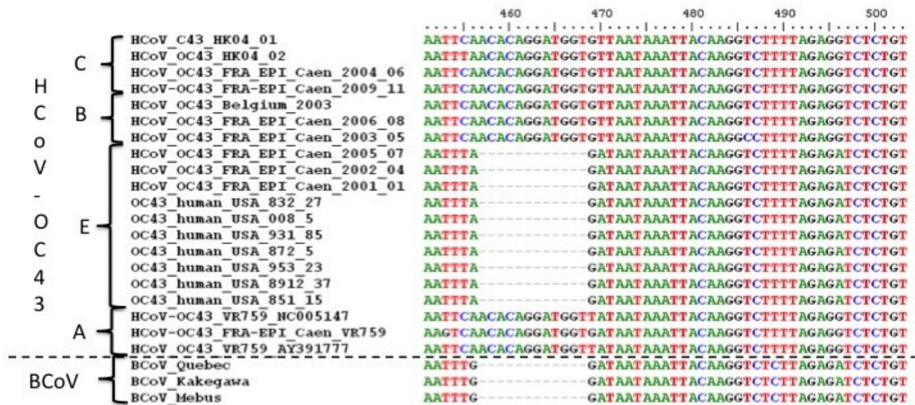
Figure 3. Alignment of some of the S genes sequences. This alignment was made using Bioedit Software version 7.2.5 (Ibis Biosciences, Carlsbad, CA, USA).
