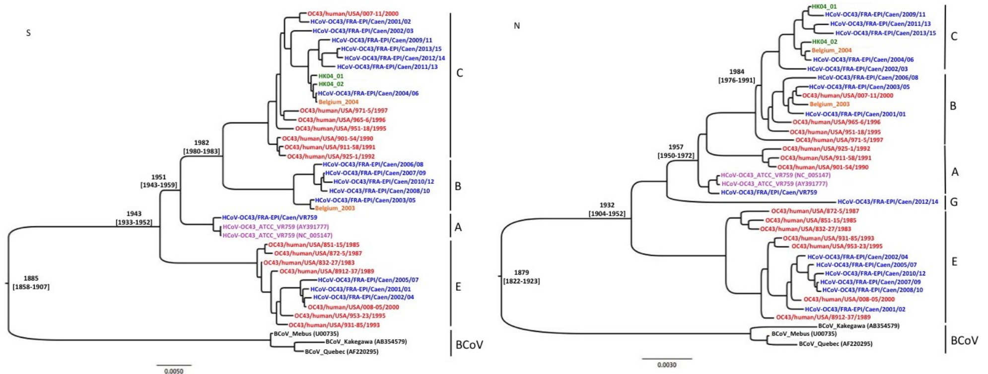
Figure 2. Results of Bayesian analysis based on S and N gene sequence data. Inferences were calculated with the one parametric coalescent model with a constant size, under the TN93+G substitution parameter, using the BEAST package (version 1.8.2) [42]. The length of MCMC was fixed at 10^8 states for S and N genes. The dates of emergence of mean clusters are indicated, associated with the 95% HPD.
