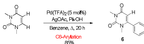
Scheme 12
