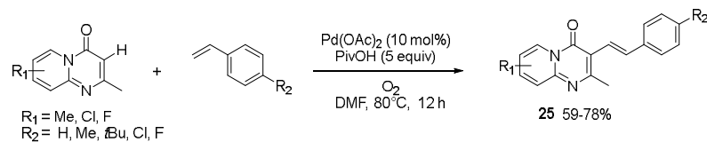
Scheme 27
