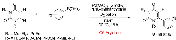
Scheme 9
