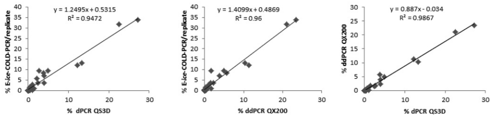
Fig. 2. Comparison of the three quantification methods for KRAS codon 12/13 in ccfDNA from colorectal cancer patients using dPCR Q53D, ddPCR QX200 and E-ice-COLD-PCR. For each sample, the genotype of the tumor DNA as determined by genotyping is shown. For E-ice-COLD-PCR the mean percentage of the detected mutation and % of the detected mutation/replicate are shown as for very low concentrations of mutated molecules not each assay will contain sufficient mutated molecules as previously shown [11]. The quantitative results for all samples are shown in three scatterplots, comparing E-ice-COLD-PCR and dPCR Q53D, E-ice-COLD-PCR and ddPCR QX200 or the two digital PCRs, respectively. They demonstrate a high linear correlation of the quantification obtained by the three technologies.
