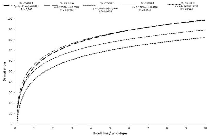
Fig. 1. Quantification by E-ice-COLD-PCR using 10 nM of blocker probes and standard curves of five cell lines (A549, SW480, LS174T, RPM1-8226 and DLD-1) with known KRAS mutations (c.34G>A, c.35G>T, c.35G>A, c.35G>C or c.38G>A, respectively) diluted in wild-type DNA to obtain mutation levels of 10%, 8%, 6%, 4%, 2%, 1%, 0.8%, 0.6%, 0.4%, 0.2%, 0.1% to 0%. All experiments were performed in sextuplicates. Standard curves were obtained by fitting data on a logarithmic scale and coefficients of regression were calculated for each mutation.
