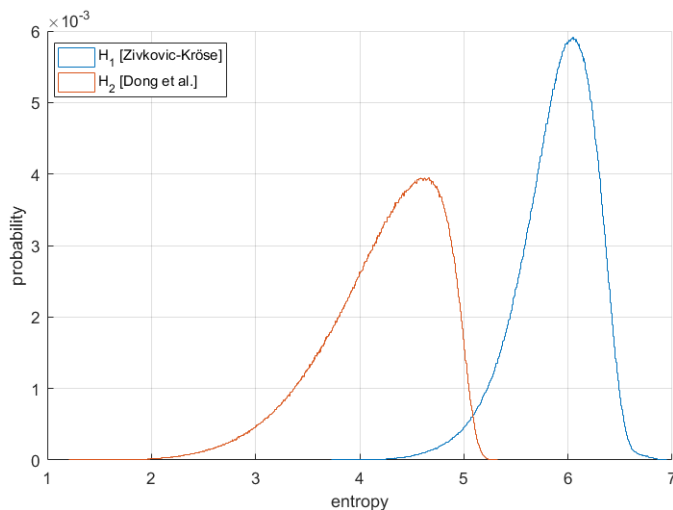
Fig. 4. Histogram distribution of entropy H_1 and H_2 extracted from the Oxford-5k dataset.
