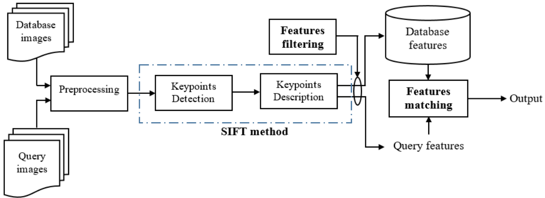
Fig. 1. The SIFT-based image matching schema with the features filtering block as a post-processing step.
