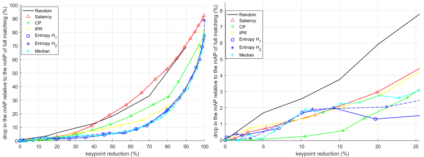
Fig. 3. Performance comparison of filtering criteria. The right figure is a zoom in for \rho \leq 25\% .
