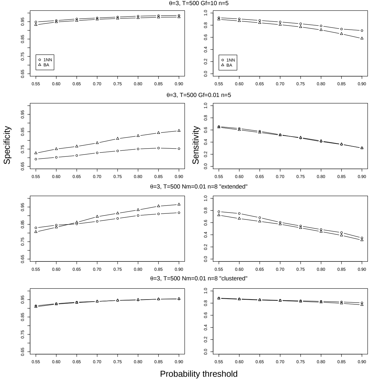
Figure 2: Robustness of coalescent-based barcoding to past population size changes and population structures. 1NN and BA are the nearest-neighbour classification and the developed Bayesian assigner with estimated mutation parameters. Results for past population size changes are presented on the first two lines, with Gf being the growth factor. A growth factor larger than one indicates a population expansion from divergence to present, whereas a growth factor smaller than one indicates a population decline. Results for population structures are presented on the last two lines, with Nm being the number of migrants exchanged between adjacent populations in one generation. BA appears robust since its performance is similar to the one of 1NN that is model-free.
