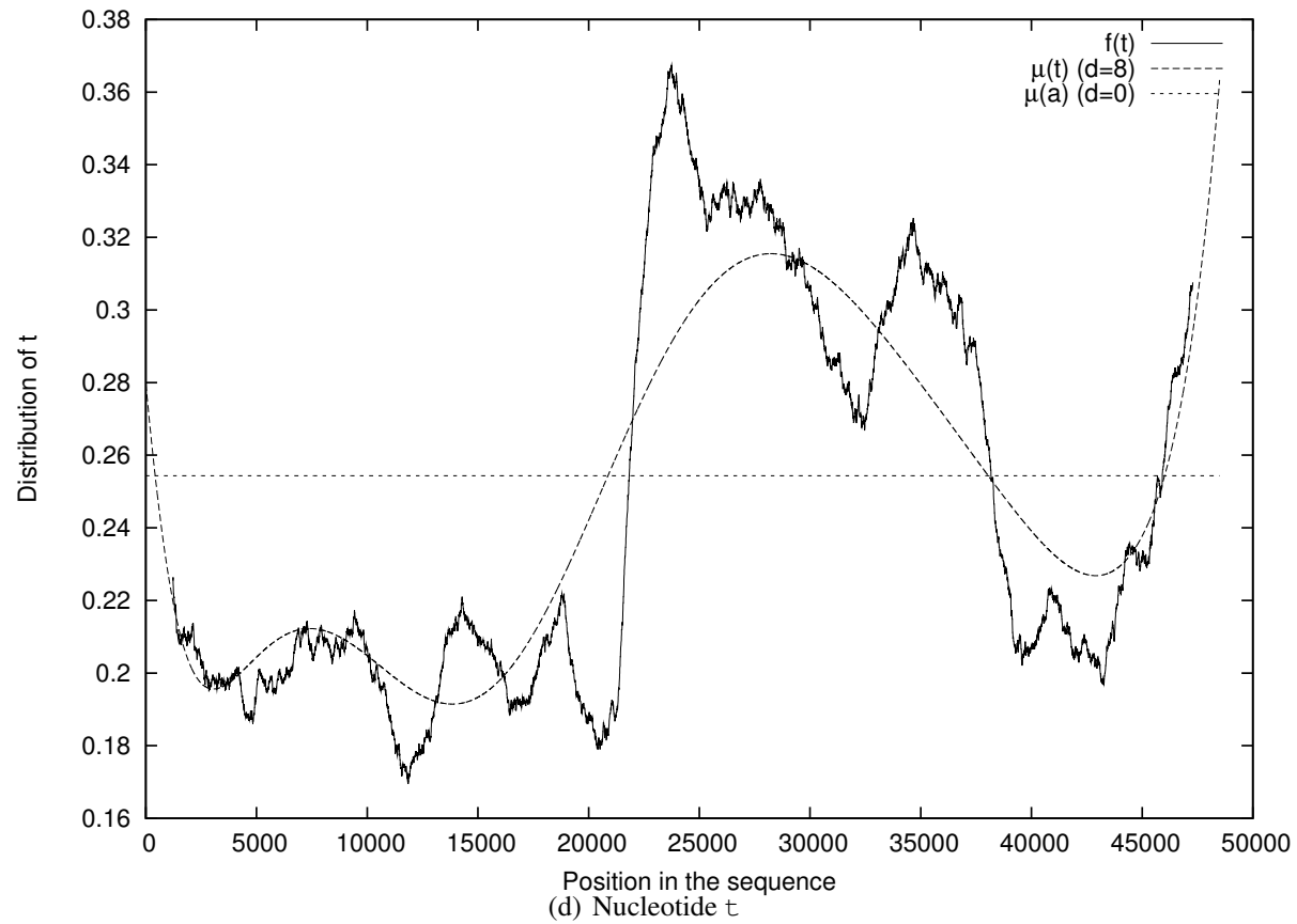
Figure 3: Frequency f and probability distribution \mu of t for degrees d = 0 and d = 8 DMM in Phage Lambda genome.
