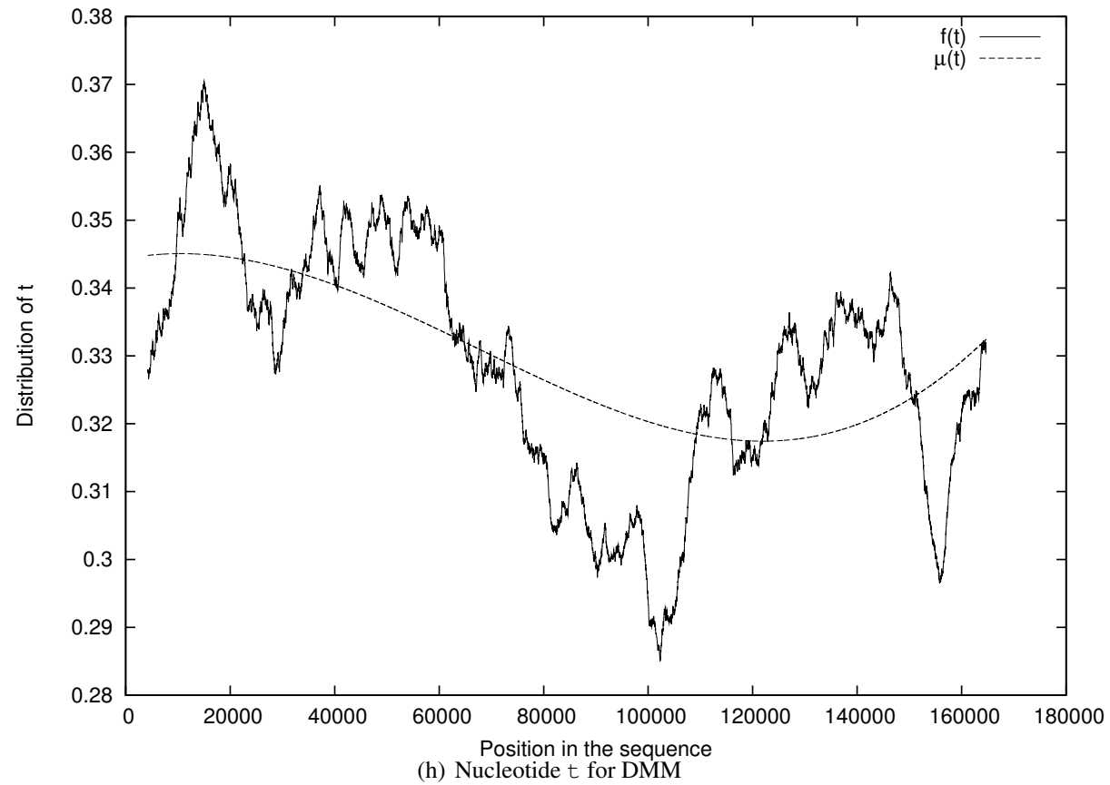
Figure 4: Frequency f and probability distribution \mu of t for a degree 3 DMM in Phage T4 genome.
