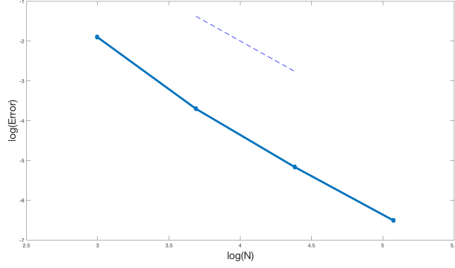
FIGURE 1. Test 1a: Convergence curve (solid line) for one order polynomial approximations ( k = 1 ). Dashed line represents a slope of order two. N denotes the number of elements.
