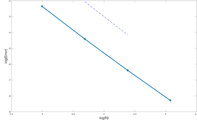
FIGURE 2. Test 1b: Convergence curve (solid line) for second order polynomial approximations ( k = 2 ). Dashed line represents a slope of order three. N denotes the number of elements.
