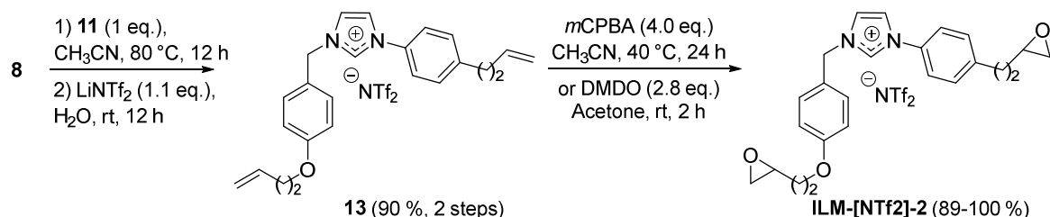
Scheme 4. Procedure synthesis of the ILM-[NTf 2 ]-2 from compounds 8 and 11
