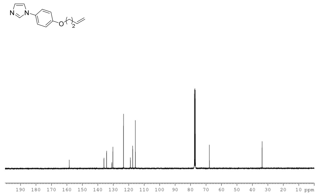
Figure S3: Analysis report for compound 3
