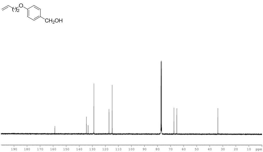
Figure S11: Analysis report for compound 10
