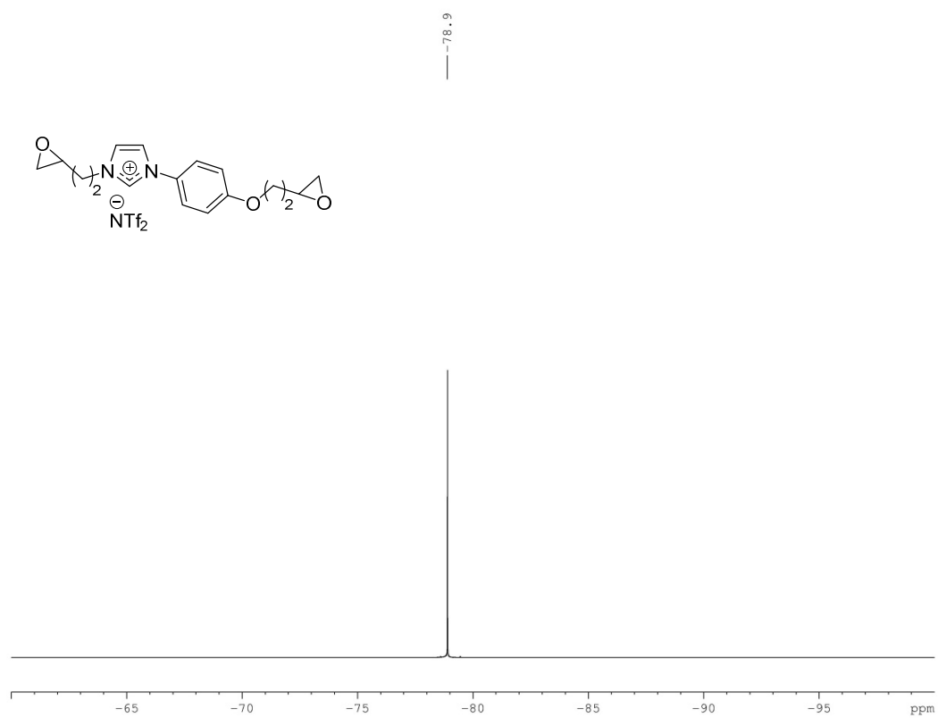
Figure S6: Analysis report for compound ILM-[NTf 2 ]-1
