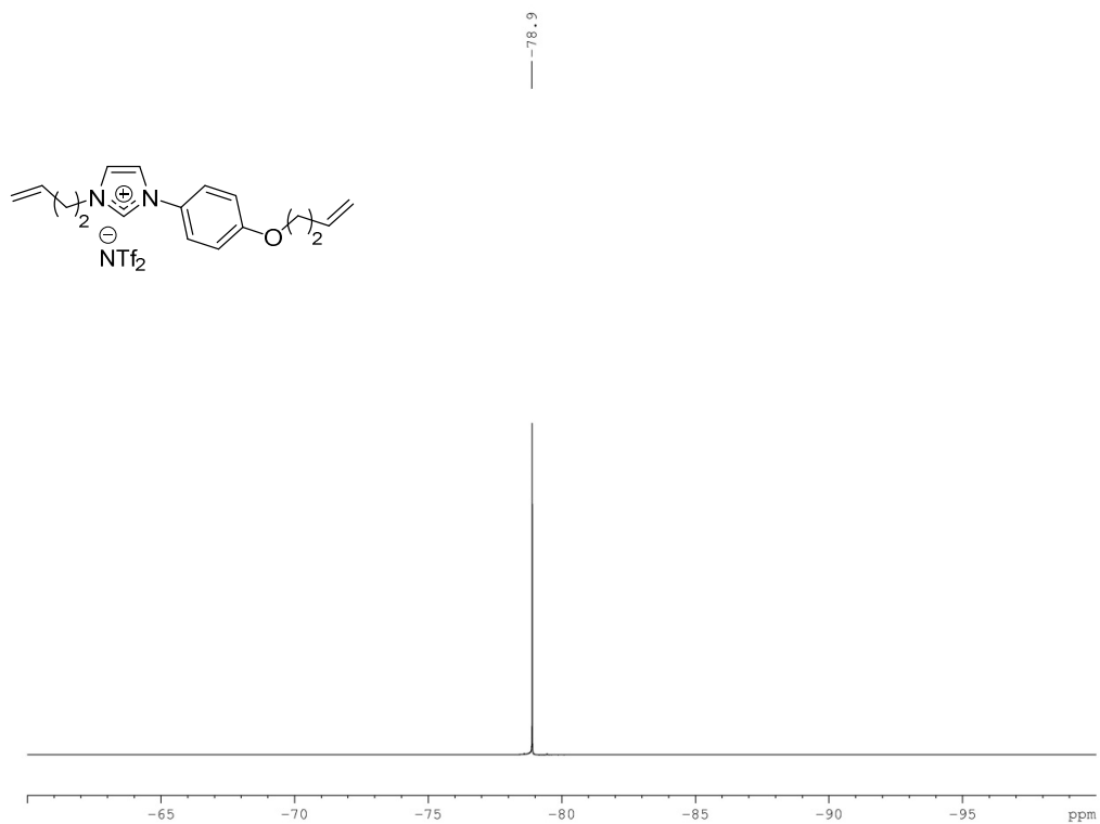
Figure S5: Analysis report for compound 5
