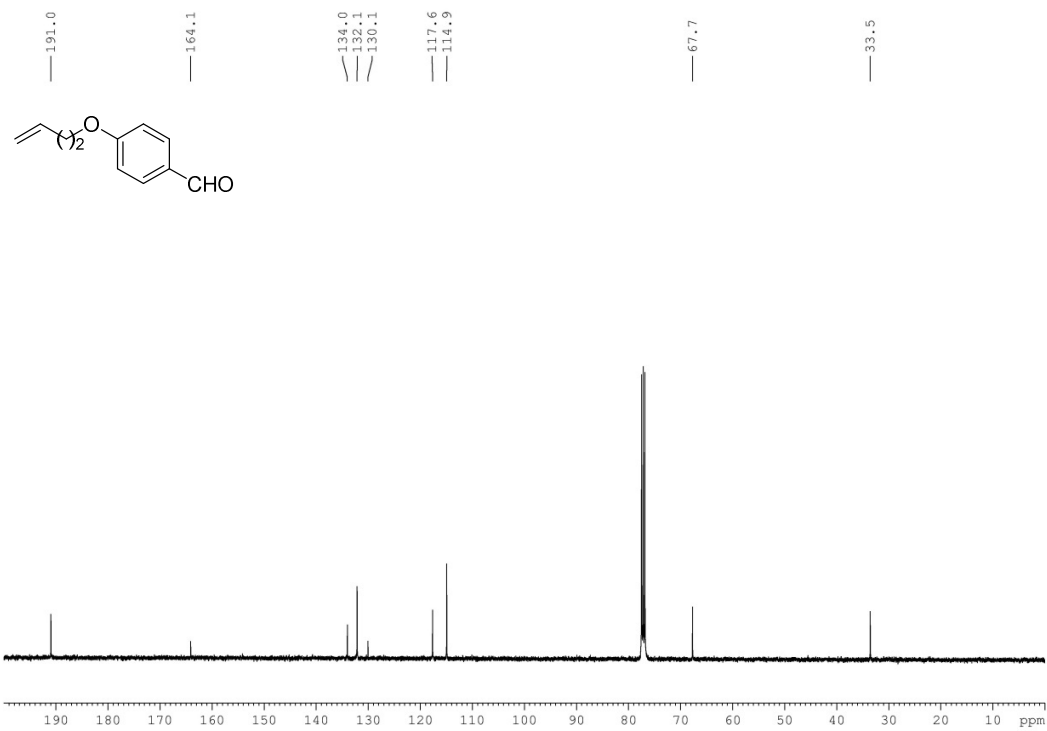
Figure S10: Analysis report for compound 9
