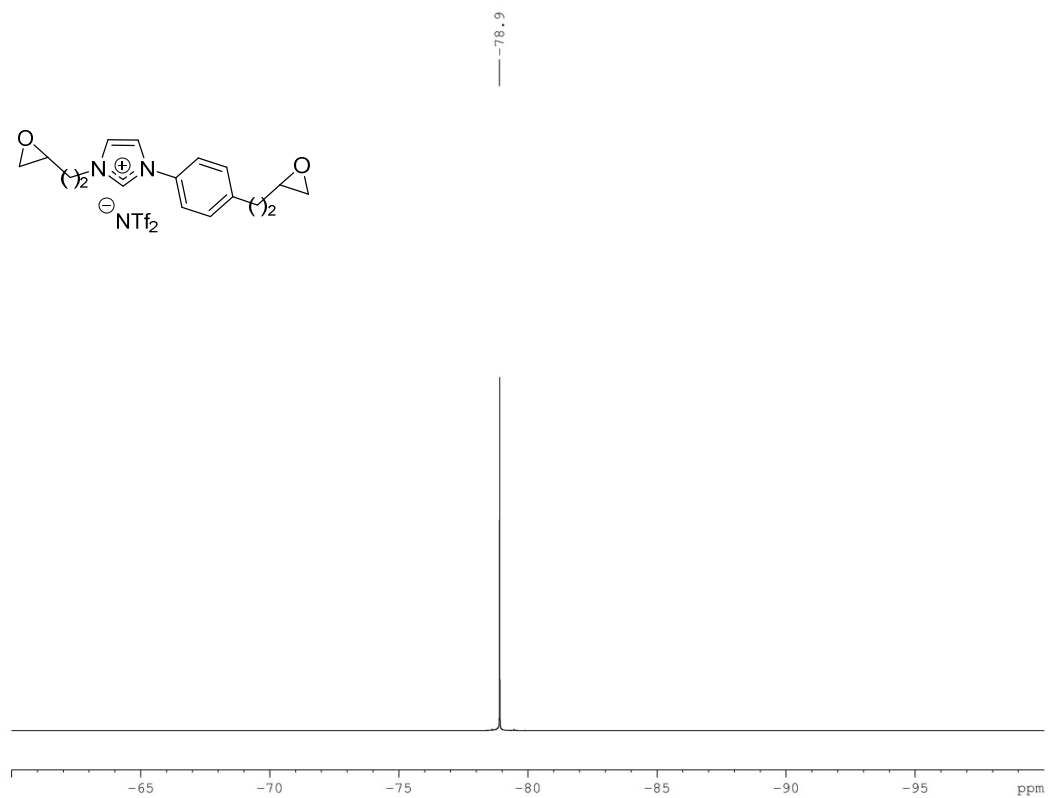
Figure S18: Analysis report for compound ILM-[NTf 2 ]-3
