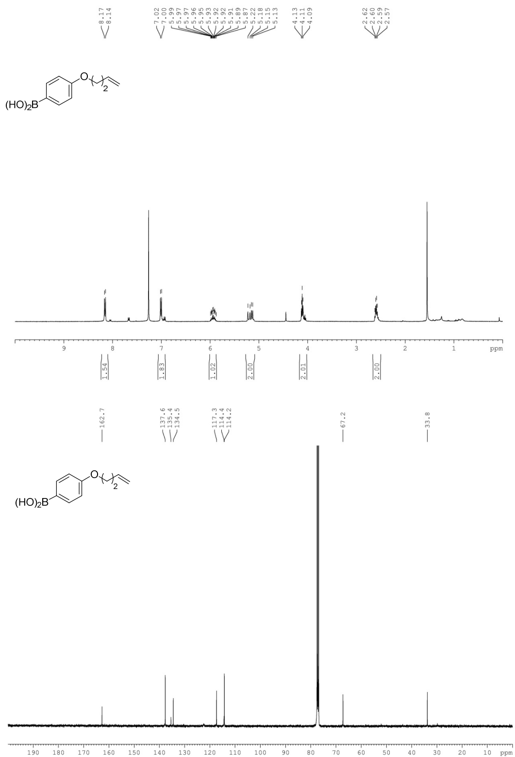
Figure S2: Analysis report for compound 2
