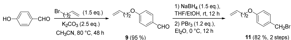
Scheme 3. Procedure synthesis of the compound 11
