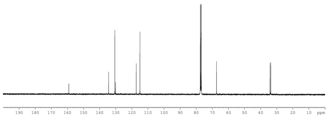
Figure S12: Analysis report for compound 11
