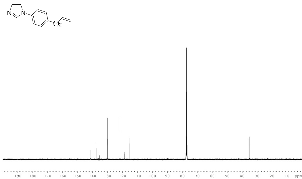
Figure S9: Analysis report for compound 8
