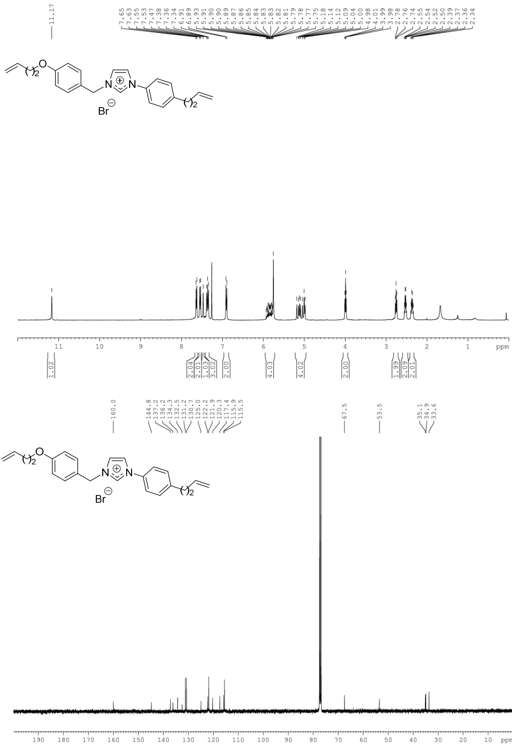
Figure S13: Analysis report for compound 12
