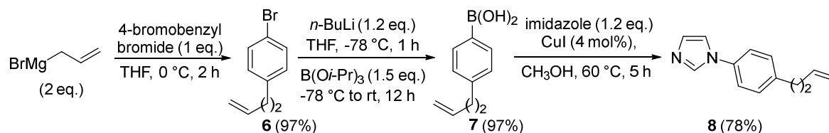
Scheme 2. Procedure synthesis of the compound 8
