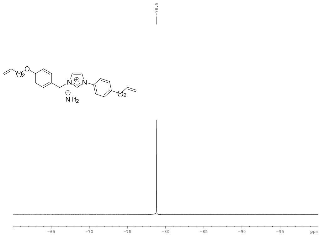
Figure S14: Analysis report for compound 13
