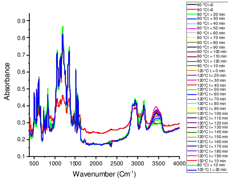
Figure S19: FTIR Spectrum of ILM-1 during curing process
