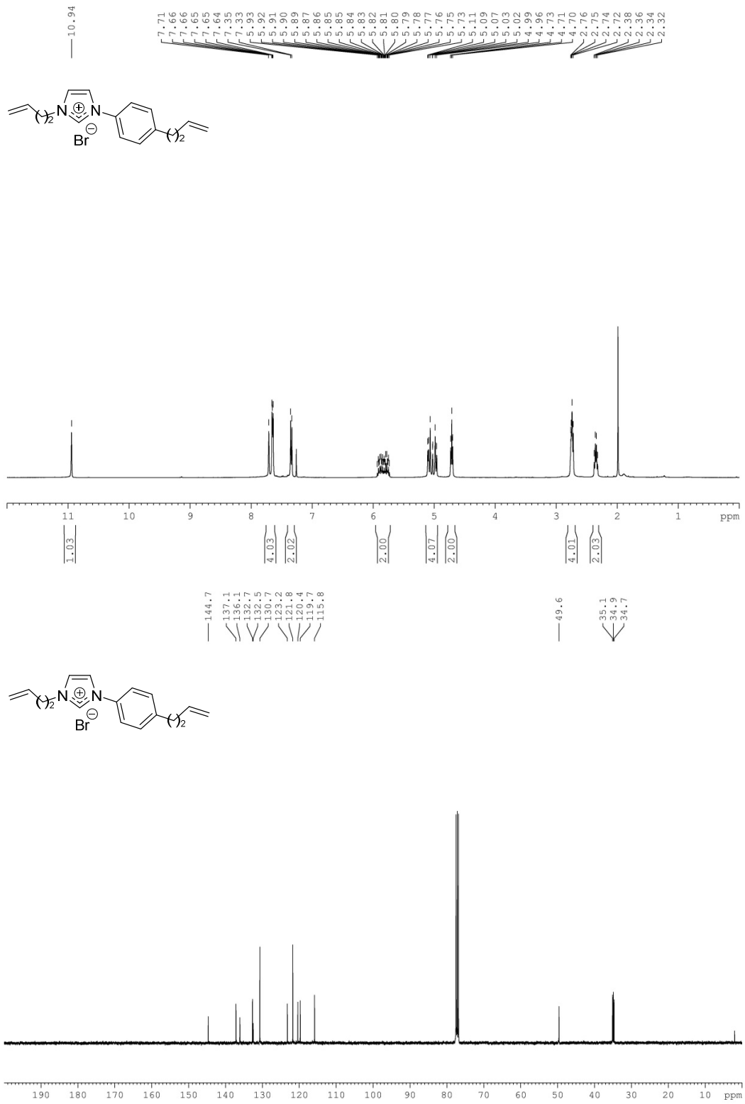
Figure S16: Analysis report for compound 14
