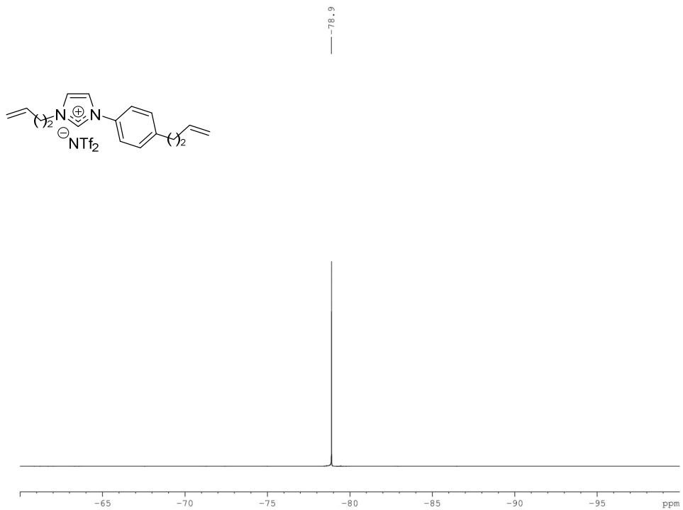
Figure S17: Analysis report for compound 15
