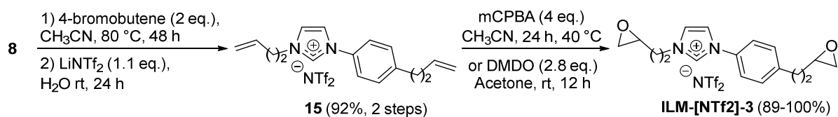
Scheme 5. Procedure synthesis of the ILM-[NTf 2 ]-2 from compound 8
