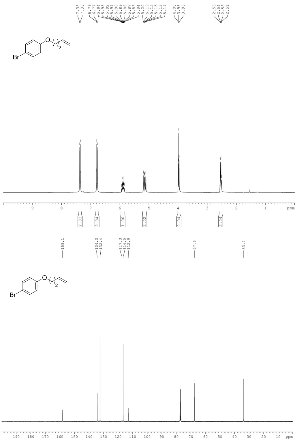
Figure S1: Analysis report for compound 1
