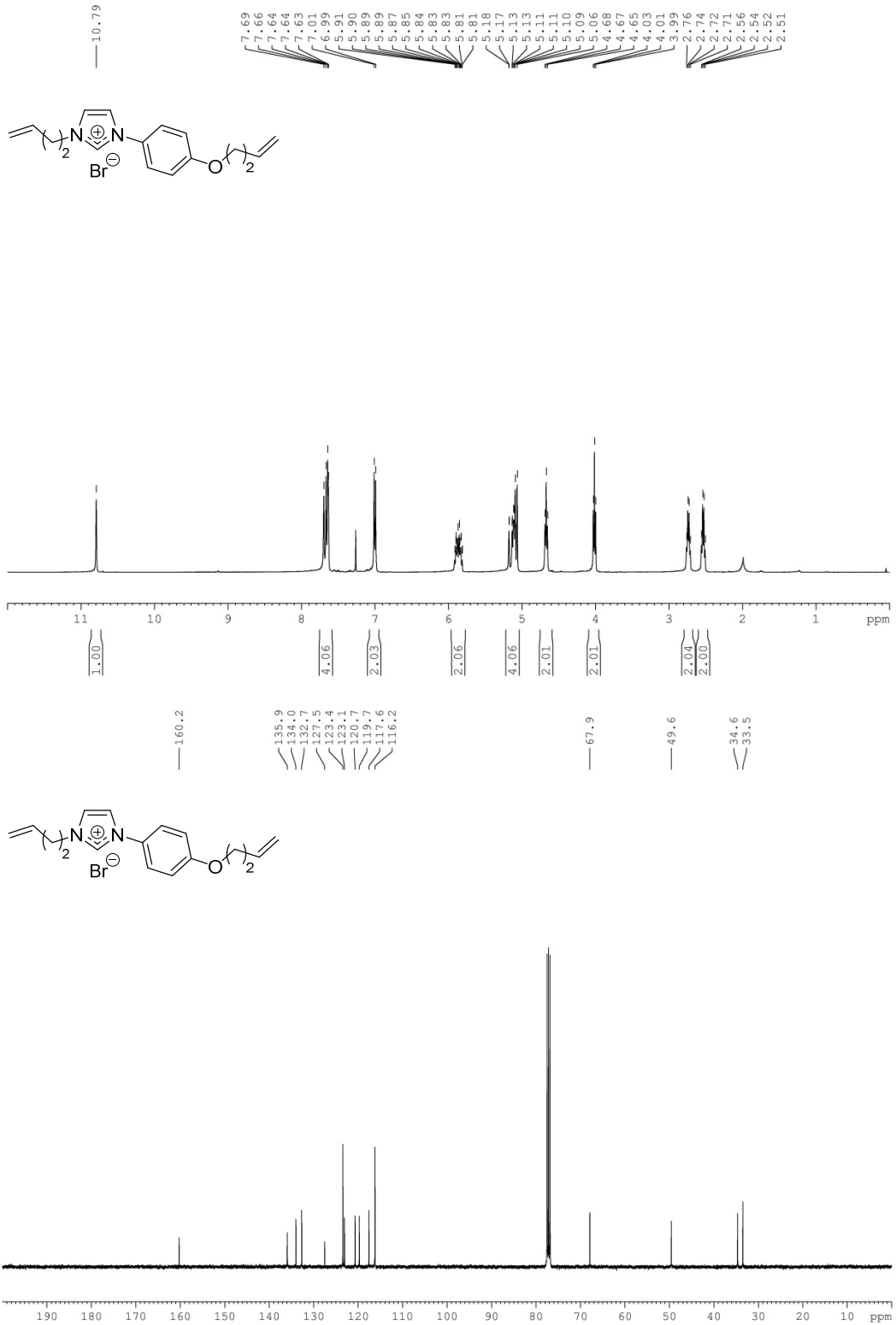
Figure S4: Analysis report for compound 4
