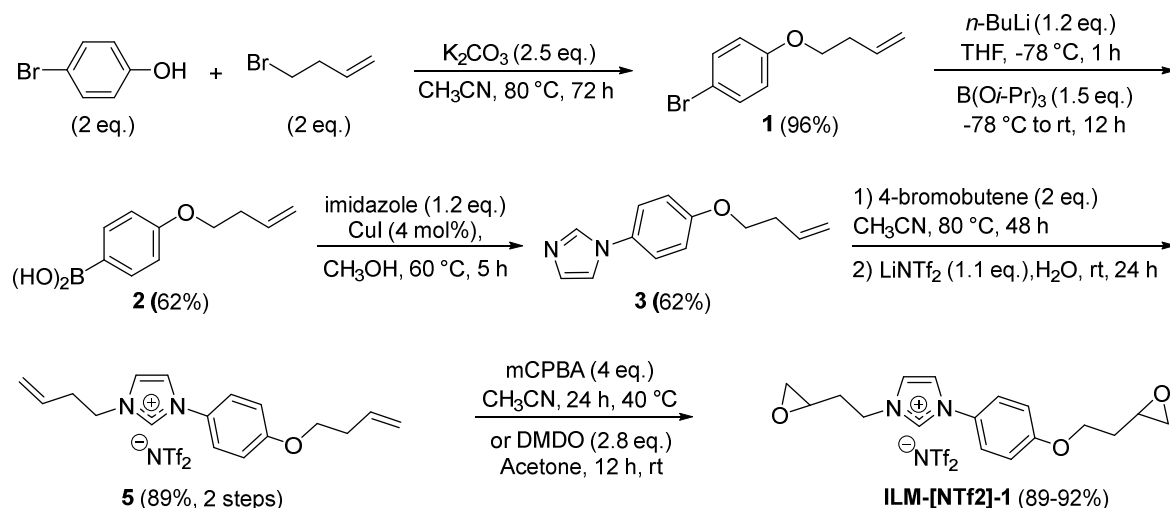
Scheme 1. Procedure synthesis of ILM-[NTf 2 ]-1
