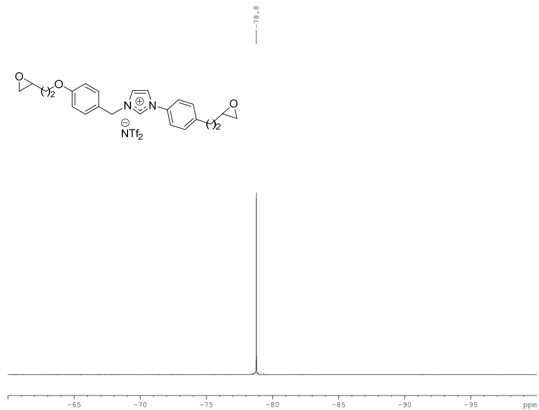
Figure S15: Analysis report for compound ILM-[NTf 2 ]-2
