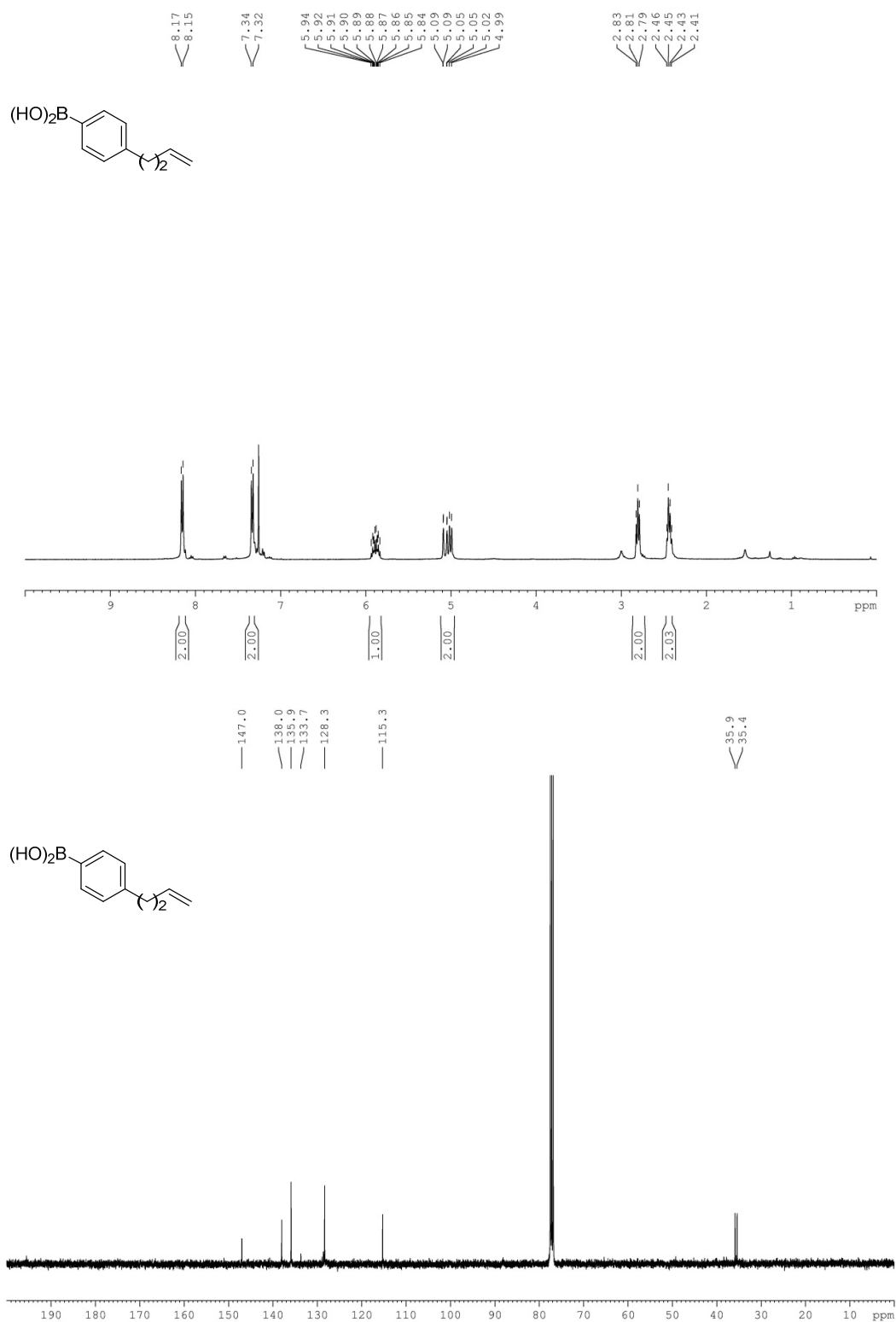
Figure S8: Analysis report for compound 7
