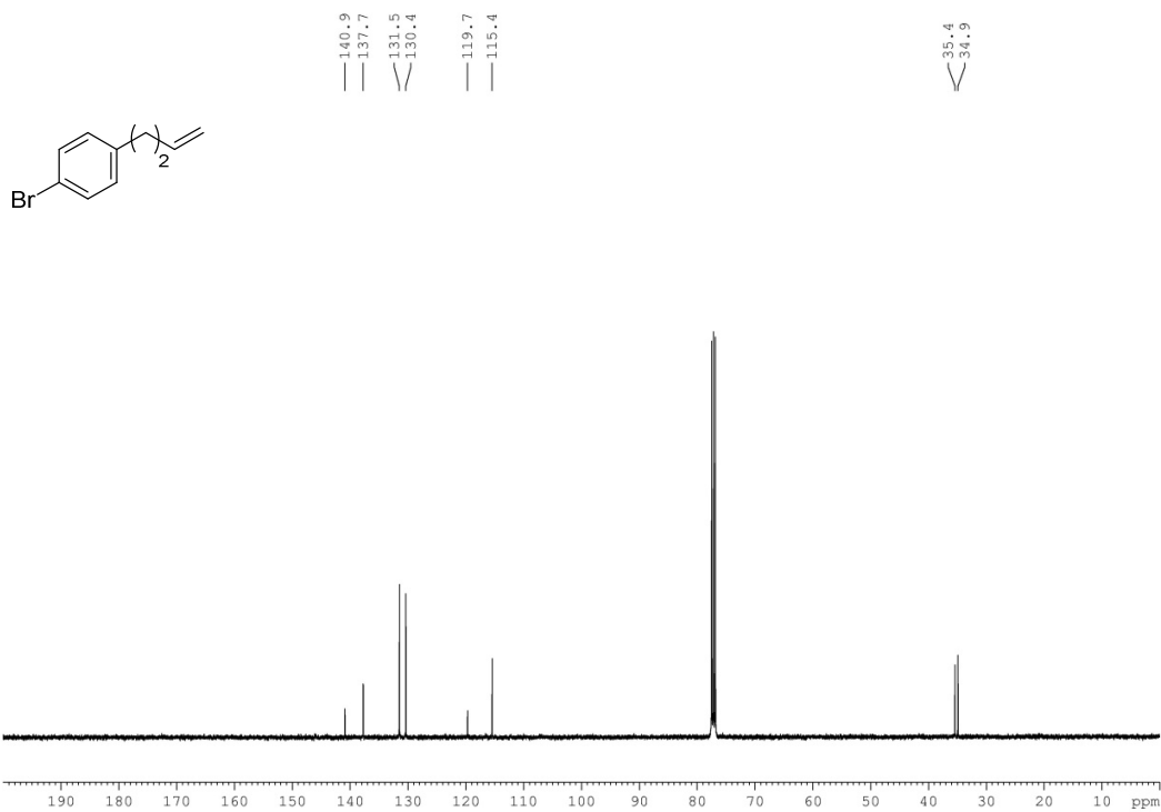
Figure S7: Analysis report for compound 6
