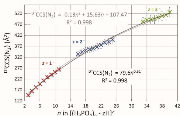
Figure 3. Graph of ^{DT}\text{CCS}(\text{N}_2) ( \text{\AA}^2 ) of phosphoric acid cluster ions vs the number of phosphoric acid molecules in the cluster. The error bars are set at 3 % of the value.
