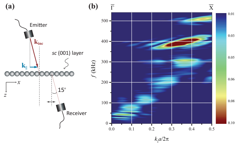
Figure 5. (a) schematic representation of the transmission configuration used to measure the guided wave response of the square monolayer of spheres. The incident and transmitted central beam axes lie on a plane containing the normal to the monolayer; the wavevector component parallel to the layer, k_{\parallel} , is along the \bar{\Gamma}\bar{X} direction of the square array; and (b) the modulus of the space-time ( x - t ) Fourier transform of the pressure transmitted in the free guided regime along the x -direction, plotted versus the reduced wavevector along the \bar{\Gamma}\bar{X} direction.
