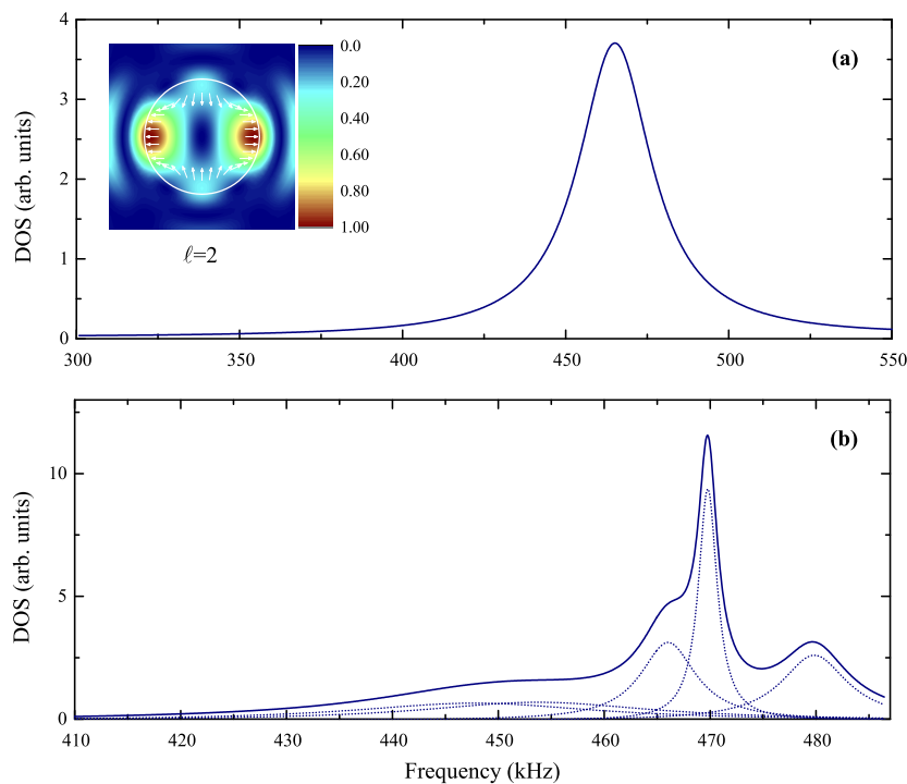
Figure 6. (a) calculated difference in the density-of-states of the elastic field for a D5N35 sphere (diameter d = 5 mm) immersed in water, with respect to the infinitely extended host medium (water), revealing an \ell = 2 five-fold resonant mode. In the inset, we give, after extraction of the incident component, the color map of the modulus of the elastic field at resonance ( f = 467 kHz), in a plane passing at the center of the sphere (incidence is assumed along the horizontal axis directed from left to right); the white arrows show the direction of the elastic field; and (b) calculated difference in the density-of-states of the elastic field for a square array of touching D5N35 spheres (diameter d = 5 mm) immersed in water, with respect to the infinitely extended host medium (water) for \mathbf{k}_{\parallel} = \frac{2\pi}{a}(0.35, 0) , revealing the splitting of the \ell = 2 five-fold resonant modes of the individual sphere to five non-degenerate modes (dotted lines).
