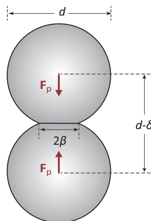
Figure A1. geometry of the problem of two elastic spheres in contact under the action of an applied compressive force.
