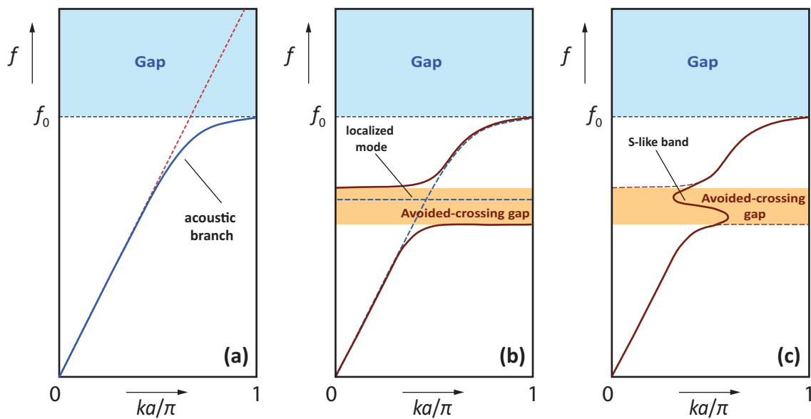
Figure A2. (a) schematic representation of the dispersion relation for a periodic mass-spring array of lattice constant a . The acoustic branch (solid line) is perfectly described, at the long-wavelength limit, by a linear dispersion corresponding to an effective-medium propagation velocity c_{eff} = \pi a f_0 (broken line), while the cut-off frequency f_0 delimits the lower frequency limit of the extended to infinity band gap (shaded area); (b) as in (a) but with the presence of a localized flat mode which, after interaction with the acoustic branch of the chain's dispersion relation, gives rise to an avoided-crossing gap (shaded area) below the cut-off frequency. Broken lines: the bands before hybridization; (c) modification of the dispersion plot shown in (b) when absorption is taken into account (see text) leading to an S-like band within the avoided-gap region, which corresponds to modes with complex wavenumber.
