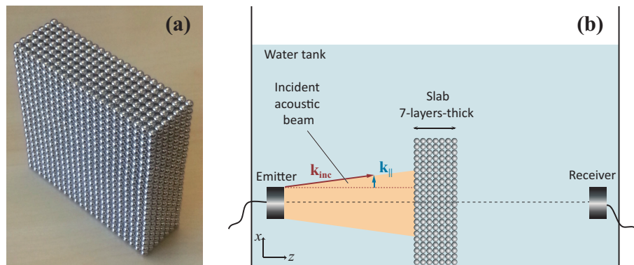
Figure 1. (a) the finite three-dimensional (3D) sc structure made of touching magnetic spheres of diameter d = 5 mm, with dimensions 11 \text{ cm} \times 11 \text{ cm} \times 3.5 \text{ cm} , before its immersion in water; and (b) schematic representation of the experimental setup. The emitter-beam angular spreading (shaded region) is characterized by a wavevector component parallel to the (001) surface of the slab, \mathbf{k}_{\parallel} , varying from zero (normal incidence) to a maximum value depending on frequency.
