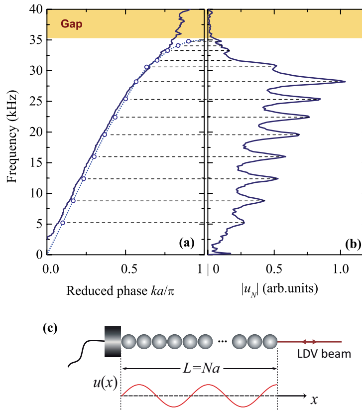
Figure 8. (a) experimental dispersion plot of a linear chain of lattice parameter a , made of N touching spheres (diameter d = a = 5 mm) deduced from the FFT phase (solid line) compared to a discrete model description represented by the pairs (k_n a/\pi, f_n) with n = 0, 1, \dots, N-1 (open symbols). The dotted line is a non-linear interpolation connecting the discrete points (k_n a/\pi, f_n) , revealing a clear propagative band ranging from 0 to 35 kHz; (b) experimental transmitted displacement field spectrum for the case of a finite chain ( N = 15 ). Horizontal dashed lines are guides to the eye, associating the frequency positions of the FP resonance peaks, f_n , to the discrete wavenumbers k_n , for the case of N = 15 spheres (see text); (c) a schematic representation of the FP resonances in the linear chain configuration with open-closed boundary conditions applied at the extremities of the chain.
