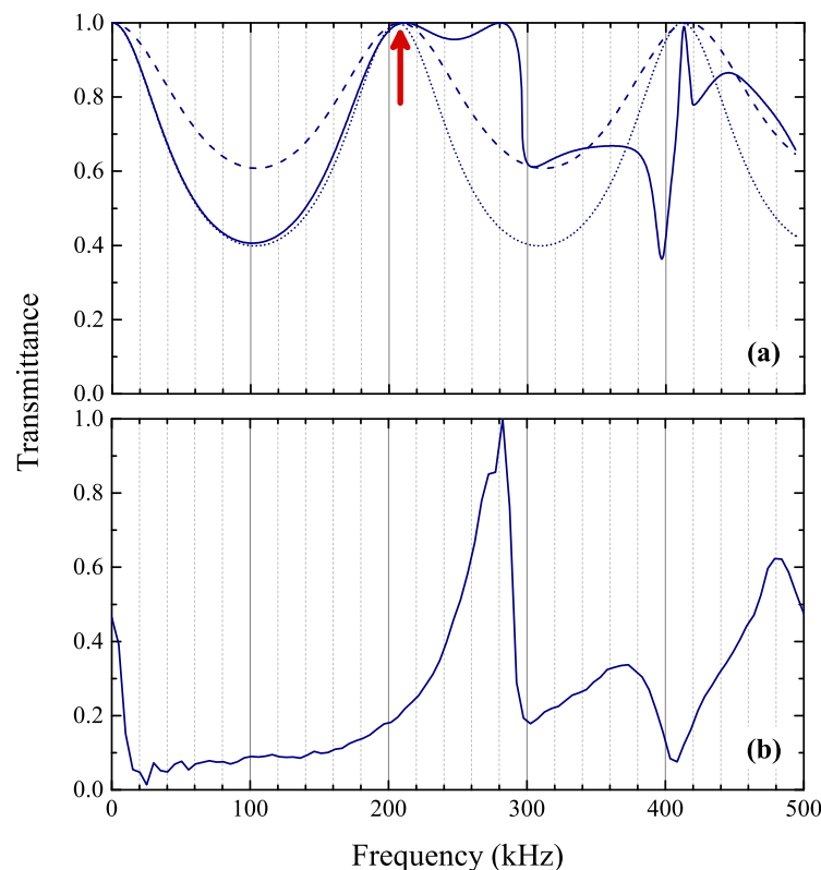
Figure 4. (a) calculated transmittance (solid line) of a plane acoustic wave through a (001) layer of D5N35 touching spheres ( a = d = 5 \text{ mm} ), immersed in water. With dashed (dotted) line we show the calculated transmittance of such a wave through an effective, homogeneous fluid plate of thickness D = 0.7a ( D = a ) with elastic parameters \bar{\rho} = 2120 \text{ kg/m}^3 ( \bar{\rho} = 2020 \text{ kg/m}^3 ) and \bar{c} = 1456 \text{ m/s} ( \bar{c} = 2060 \text{ m/s} ). The red arrow indicates the position of the first FP resonance; and (b) the corresponding measured transmitted pressure of a (001) layer of spheres excited by an immersion transducer beam.
