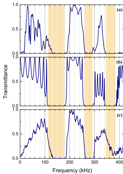
Figure 2. (a) measured transmittance of an acoustic beam incident on the seven-(001)-layers thick slab of the 3D sc crystal immersed in water; (b) calculated transmittance of a longitudinal plane wave incident normally ( \mathbf{k}_{\parallel} = \mathbf{0} ) on the structure; and (c) normalized sum of the calculated transmittances over several \mathbf{k}_{\parallel} = \frac{\pi}{a}(q, 0) components, with q varying from 0 to \frac{2}{3} with a step of \Delta q = \frac{1}{30} . Shaded regions show gap positions for (b) to guide the eye.
