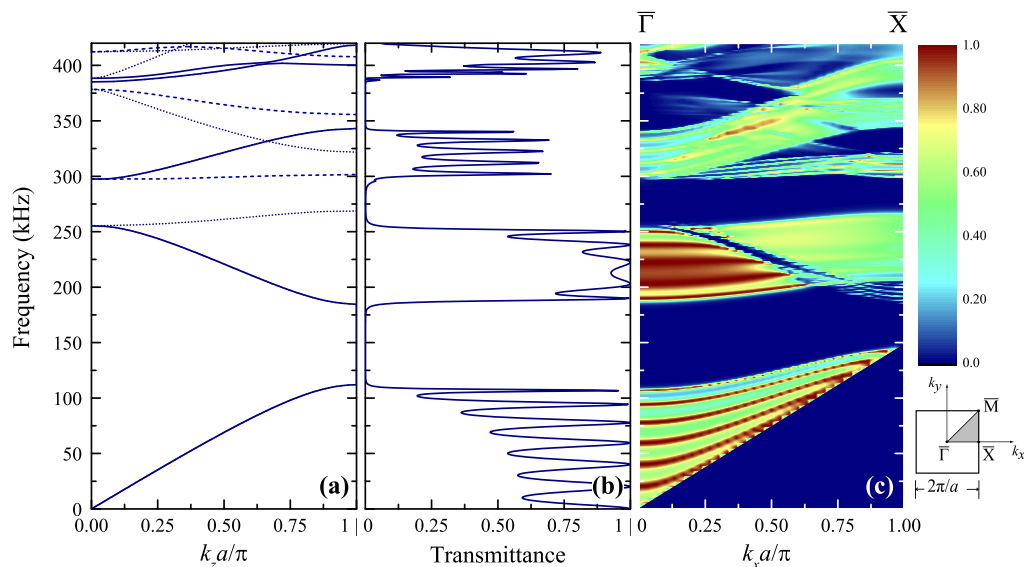
Figure 3. (a) calculated frequency band structure for the 3D cubic crystal of touching D5N35 spheres (lattice parameter a = d = 5 mm), immersed in water, along the direction [001] ( \mathbf{k}_{\parallel} = \mathbf{0} ). Solid, dotted and dashed lines denote, respectively, active non-degenerate bands (symmetry \Delta_1 ), inactive non-degenerate bands (symmetry \Delta_1' , \Delta_2 , \Delta_2' ) and inactive double degenerate bands (symmetry \Delta_5 ); (b) the corresponding transmittance of a longitudinal plane wave incident normally on a seven-(001)-layers thick slab of the crystal; and (c) color map of the transmittance spectra along the \Gamma\bar{X} direction ( \mathbf{k}_{\parallel} = (k_x, 0) ) of the surface Brillouin zone shown in the margin.
