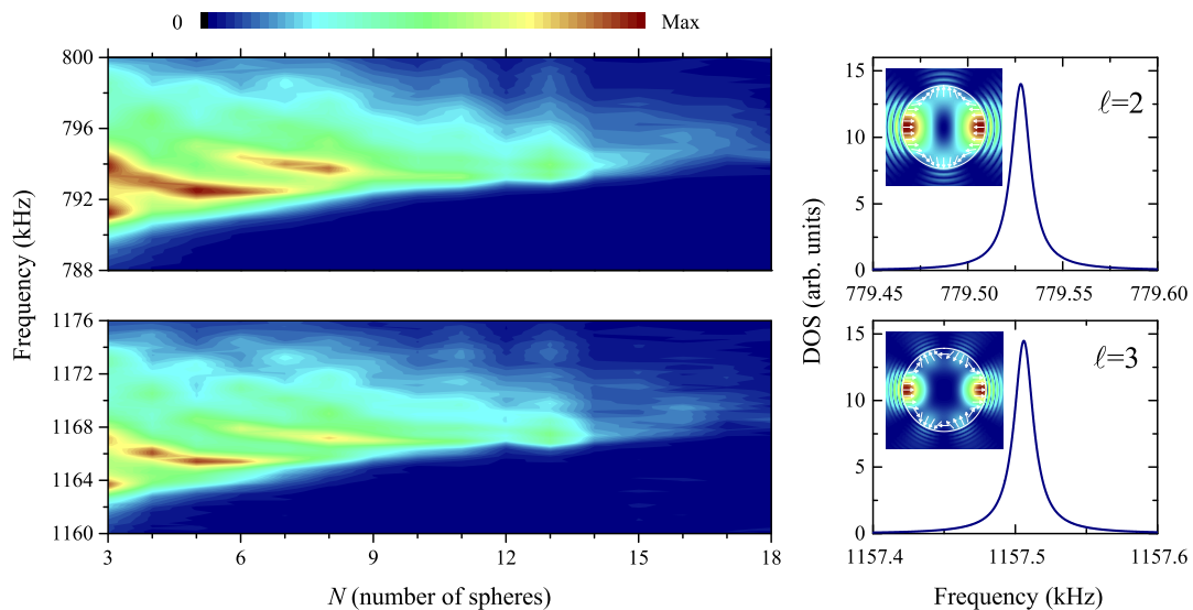
Figure 10. (left): color map of the transmitted displacement field measured at the end of a chain made of N D3N42 magnetic spheres ( d = 3 mm), as a function of frequency and number of spheres. Two narrow localized bands are observed, originating from \ell = 2 (top) and \ell = 3 (bottom) resonance modes of the individual sphere; (right), the corresponding DOS calculations for one sphere, together with the elastic field on resonance, at a cut passing at the center of the sphere (incidence is considered from left to right).
