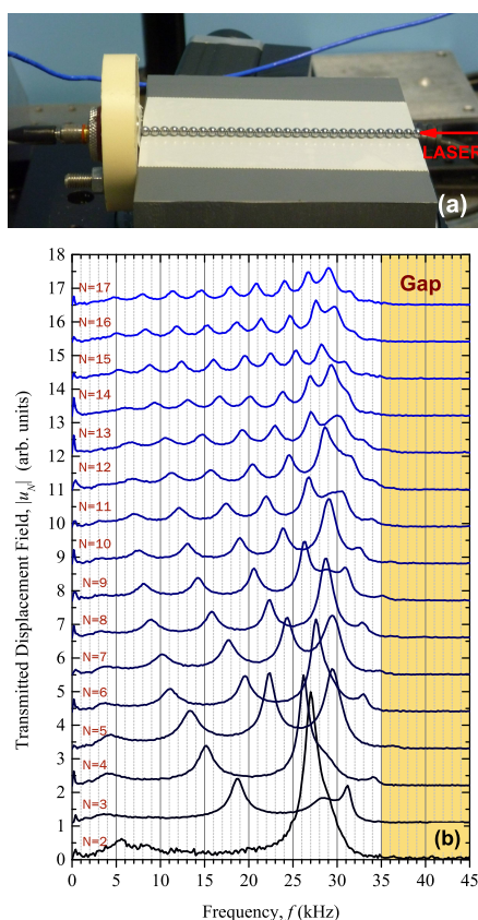
Figure 7. (a) chain of N metallic spheres of diameter d = 5 mm, excited by a longitudinal transducer (left) with the transmitted signal recorded at the end of the chain through LDV (right); (b) the modulus of the transmitted displacement field measured at the end of the chain, |u_N(f)| , as a function of frequency f , for various chain lengths, L = Nd . The different spectra are displaced vertically to improve visibility.
