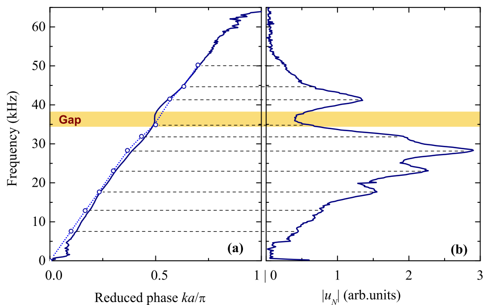
Figure 9. (a) experimental dispersion plot of a linear chain of lattice parameter a , made of N touching spheres (diameter d = a = 3 mm); (b) experimental transmitted displacement field spectrum for the case of a finite chain ( N = 15 ). All symbols, methods and analysis follow the same scheme as the one used in Figure 8.
